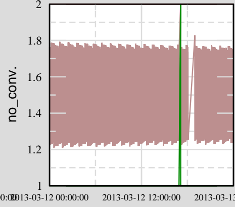
Ch 13: H0:PEM-LAB_DST1_MODE
