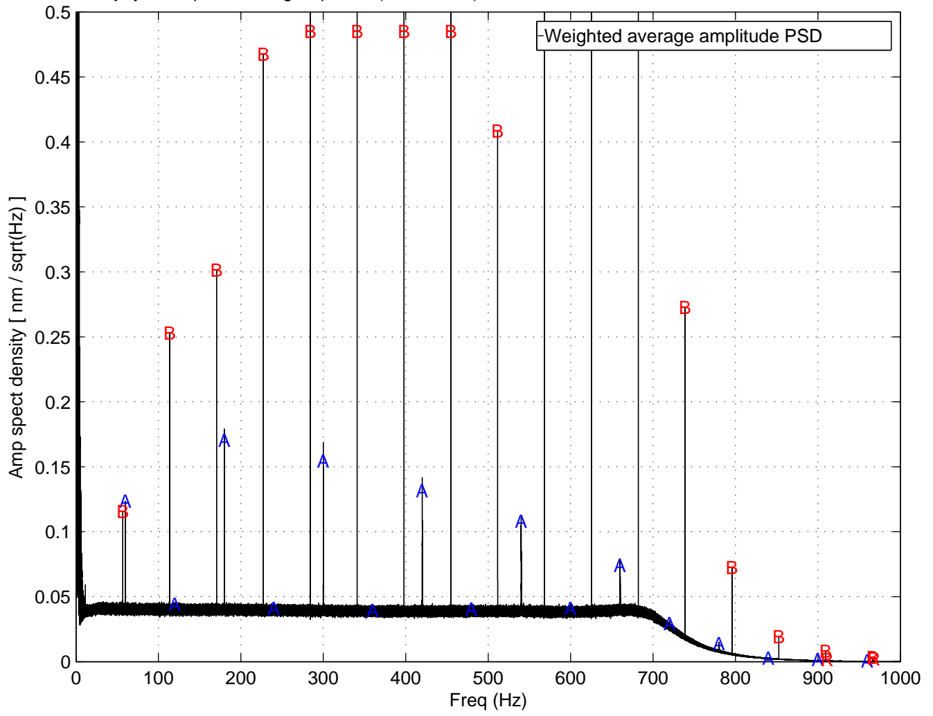
july16+sept13 Average Spectra (0-1000 Hz) - H2_SUS-ETMY_L1_OSEMINF_LL_IN1_DQ
