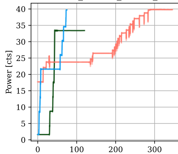
H1:ASC-X_TR_B_NSUM_OUT16
