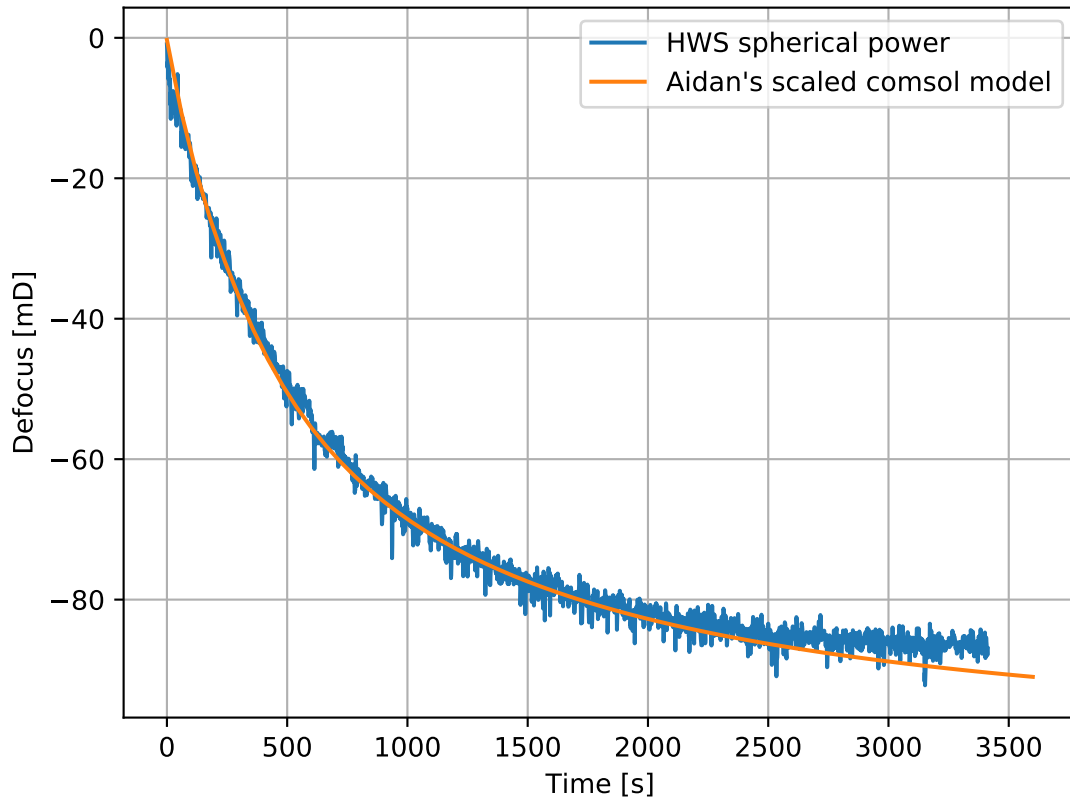
Fitting HWS spherical power, 96 mW absorbed power
