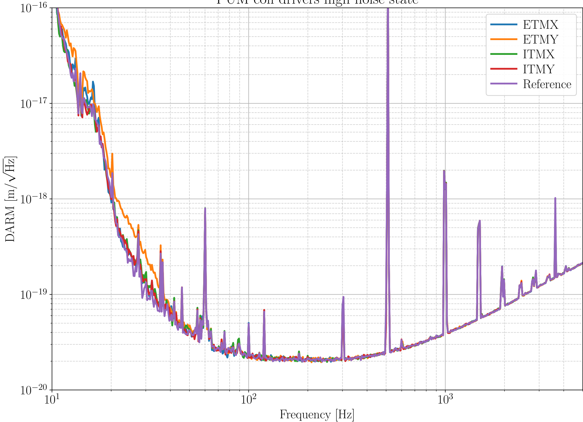
PUM coil drivers high noise state
