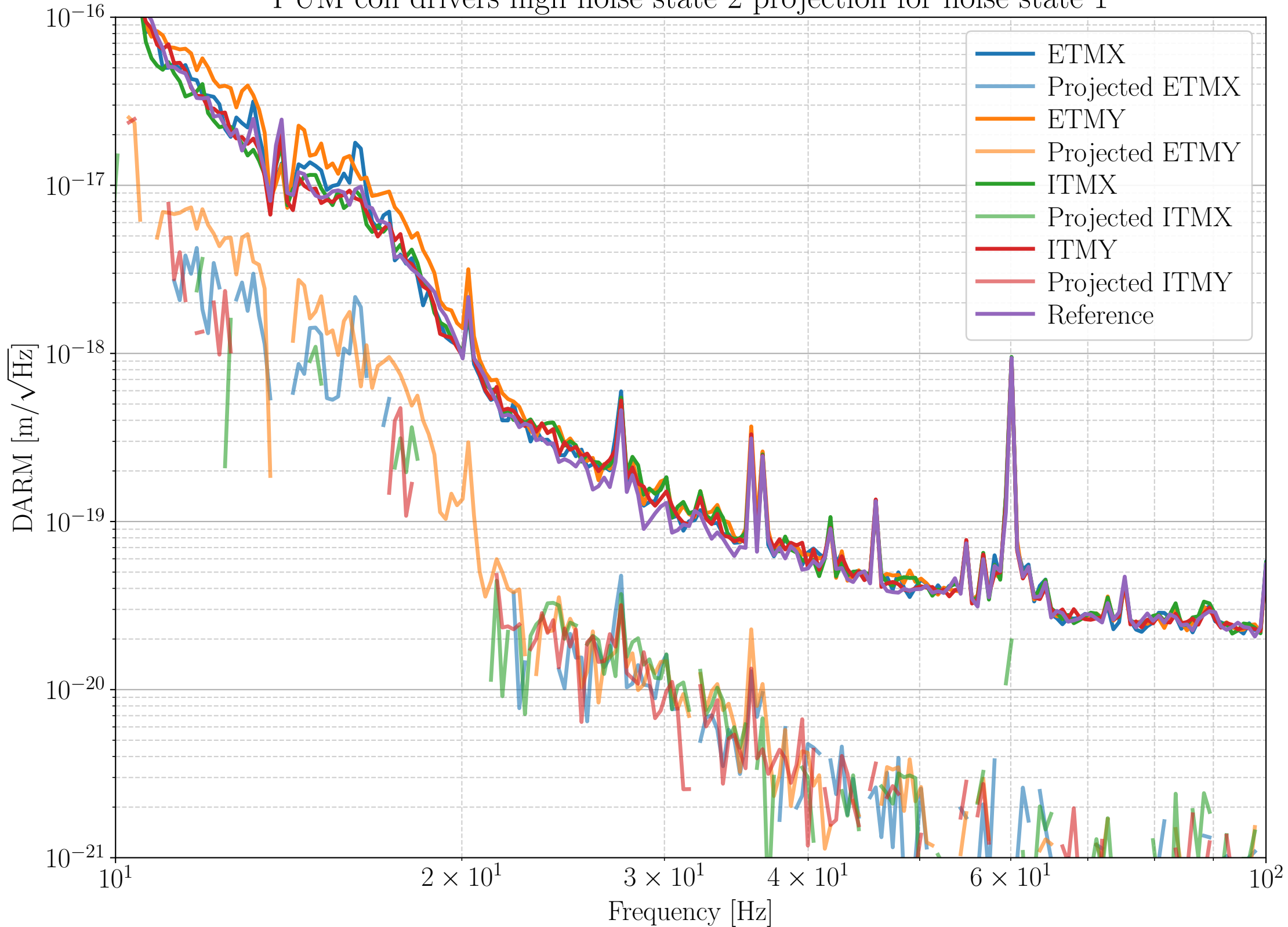
PUM coil drivers high noise state 2 projection for noise state 1
