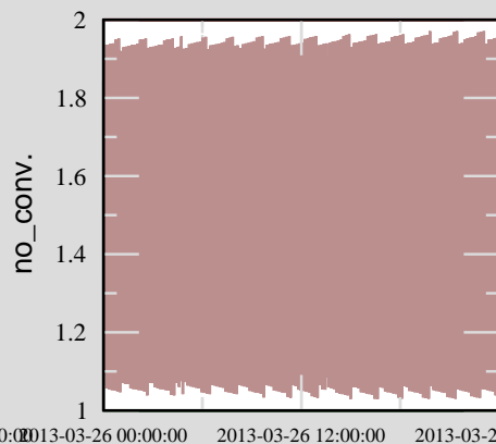
Ch 7: H0:PEM-LVEA_DST14_MODE
