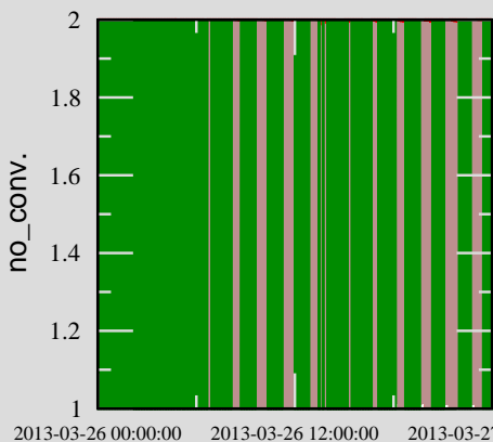
Ch 3: H0:PEM-LVEA_DST5_MODE
