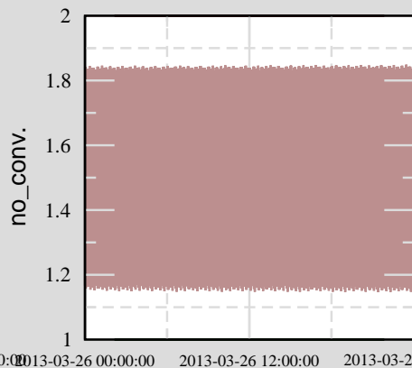
Ch 9: H0:PEM-LVEA_DST16_MODE
