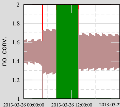
Ch 2: H0:PEM-LVEA_DST4_MODE
