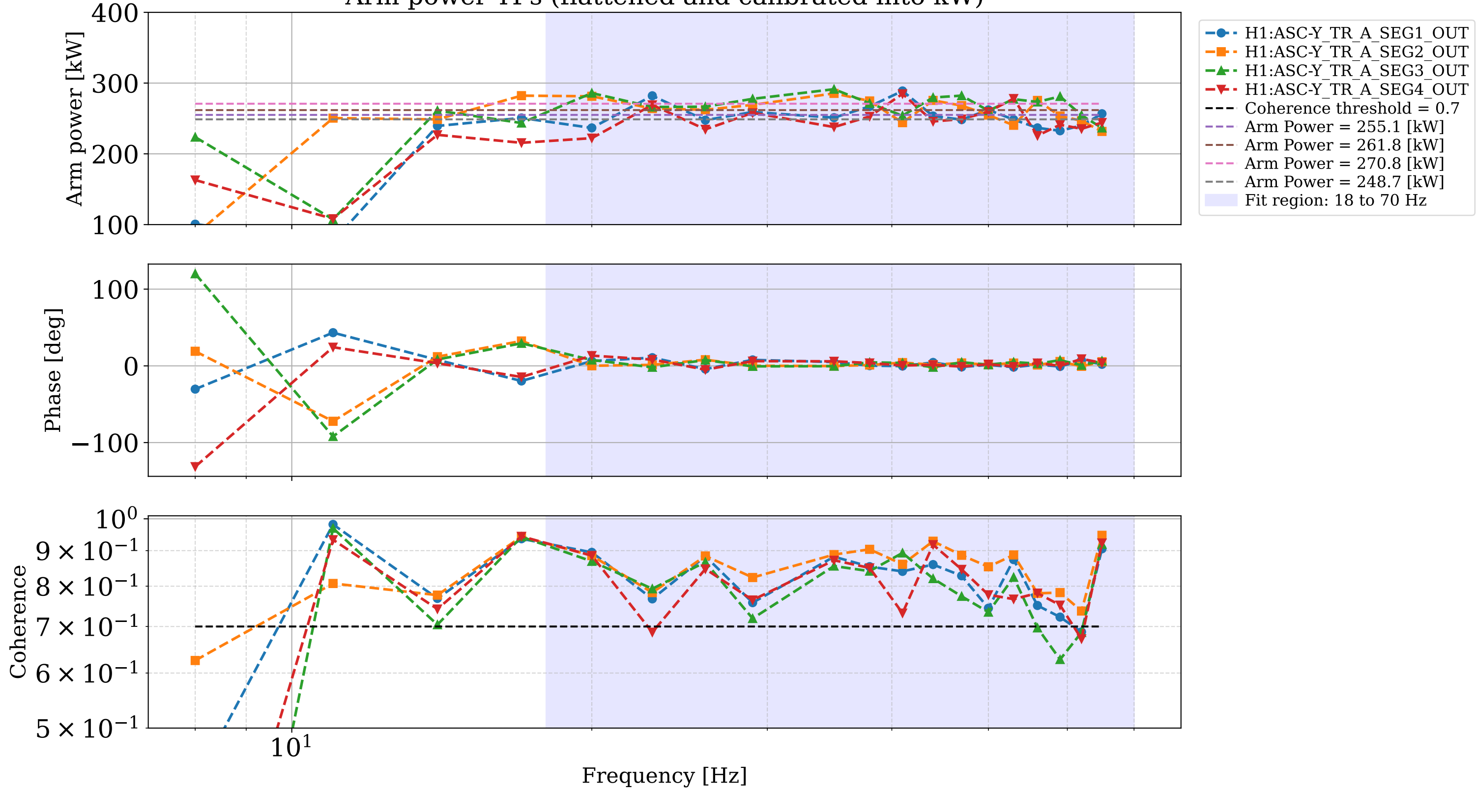
Arm power TFs (flattened and calibrated into kW)
