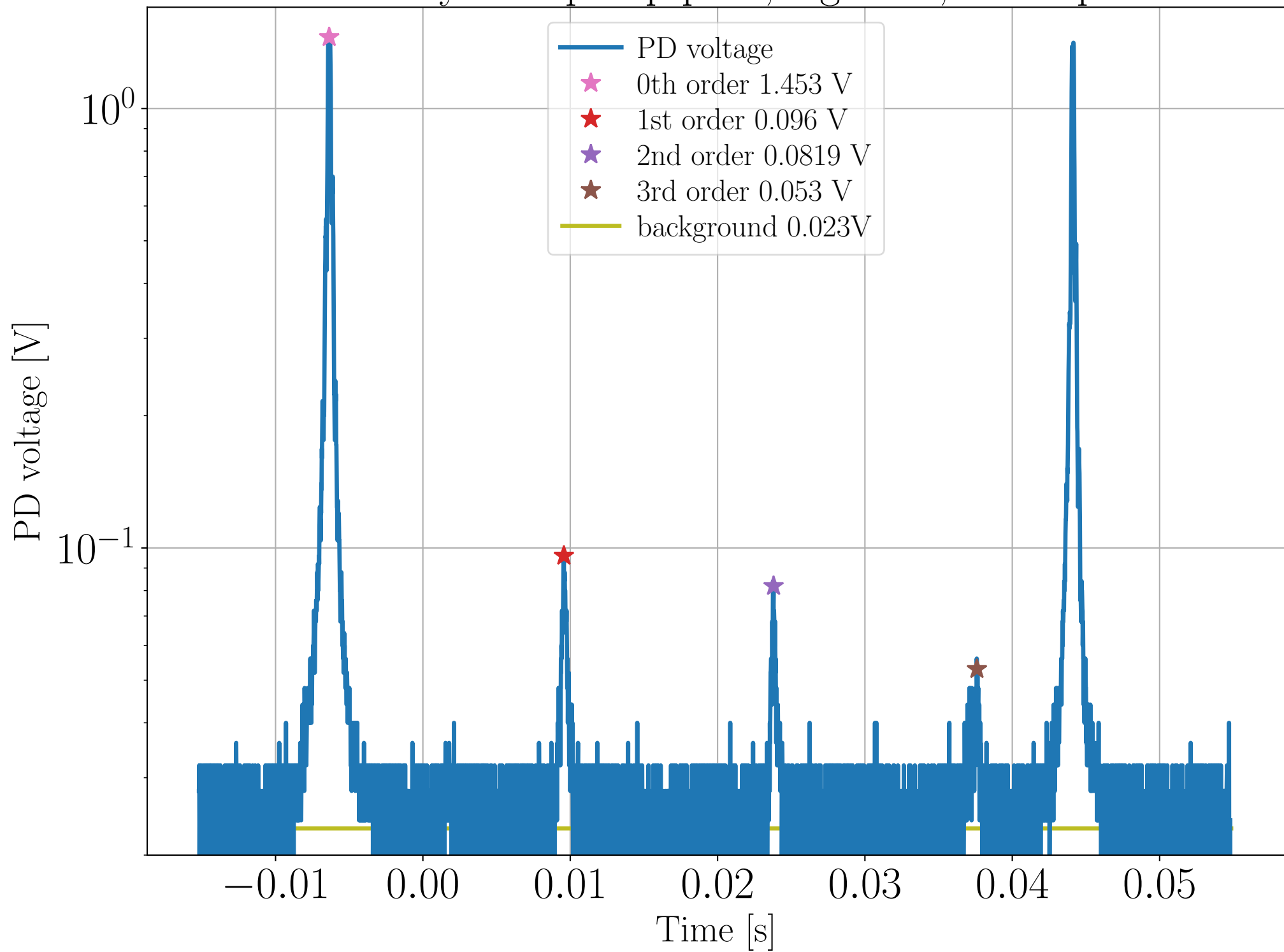
OPO cavity scan pump path, log scale, HOM power
