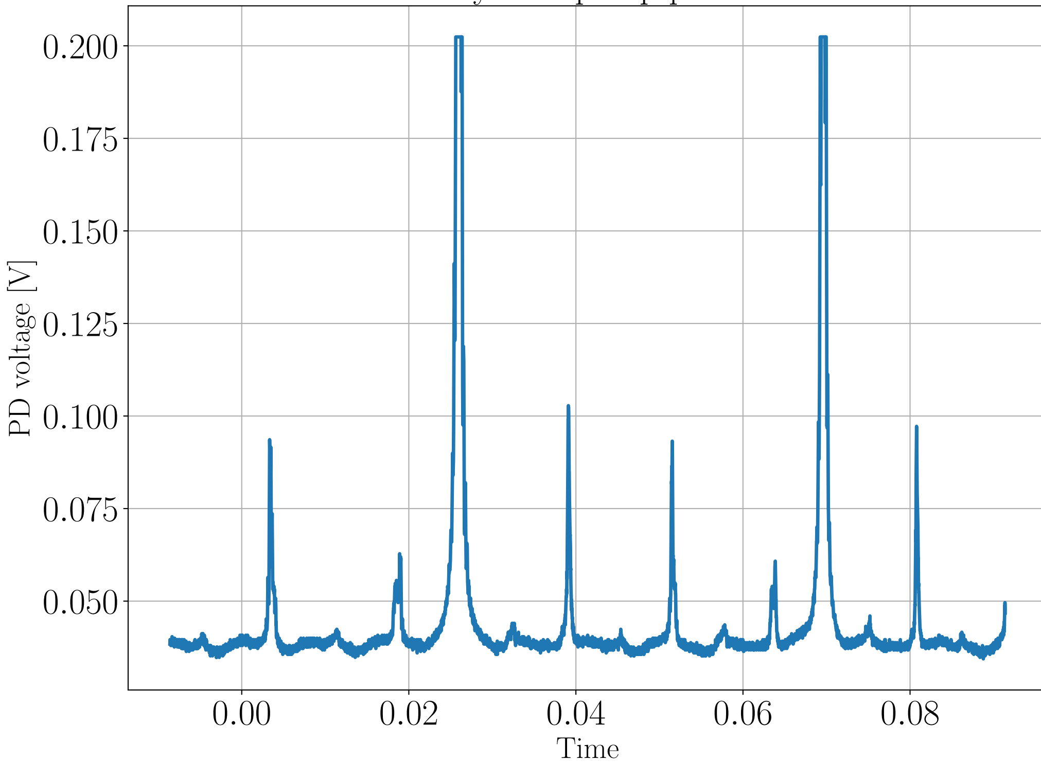
OPO cavity scan pump path zoomed
