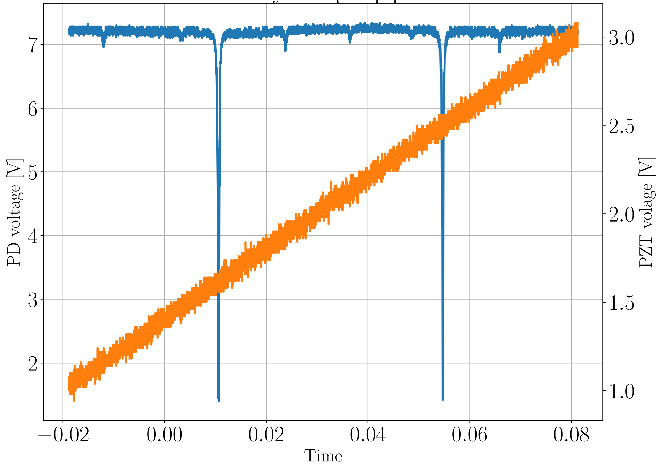
OPO cavity scan pump path refl
