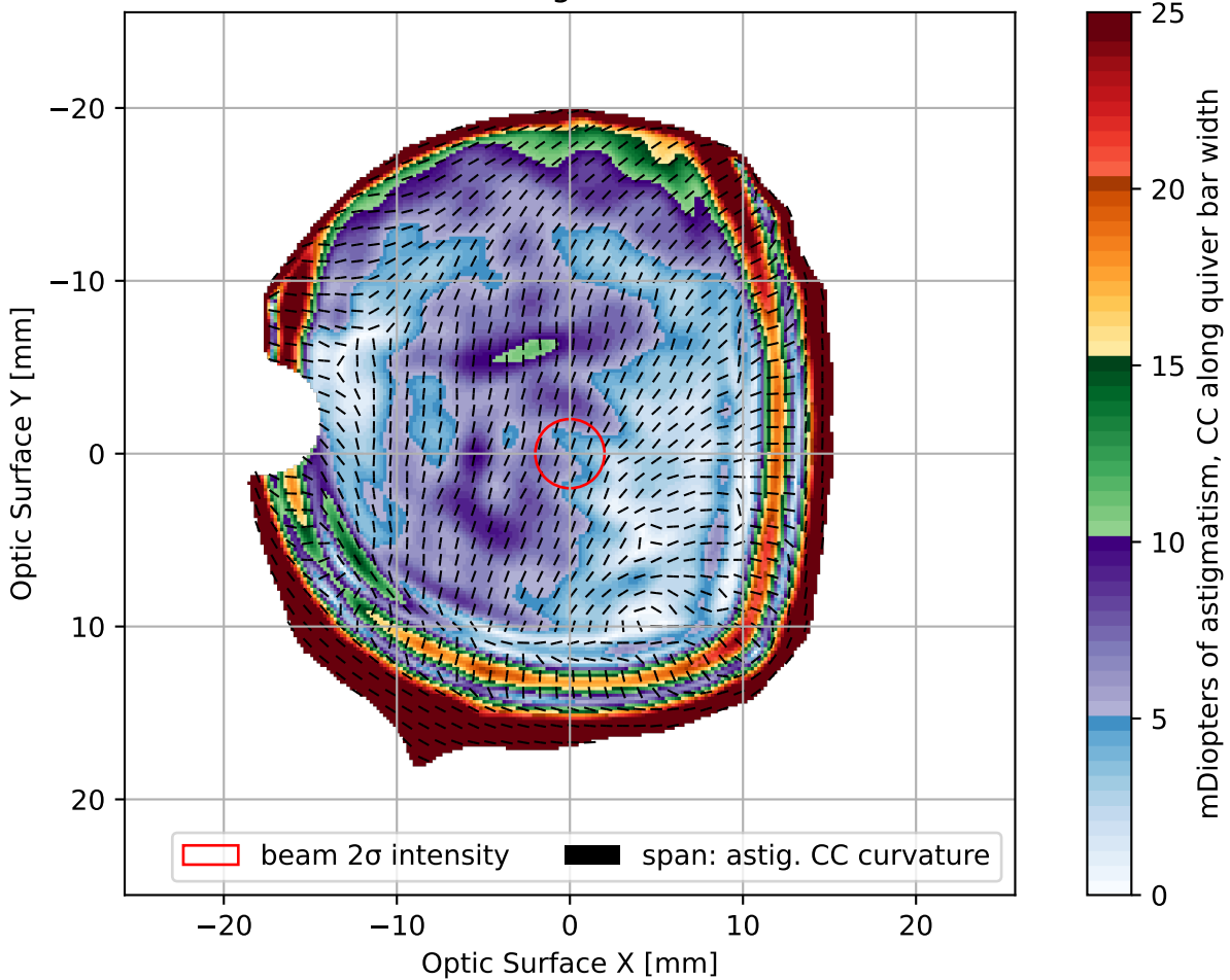
ZM4-SN1-00V astigmatism field in mD
