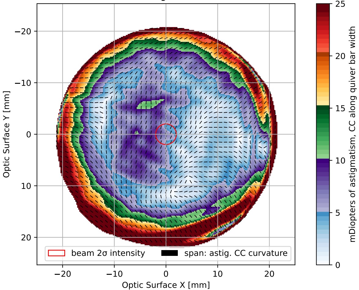
ZM4-SN1-50V astigmatism field in mD
