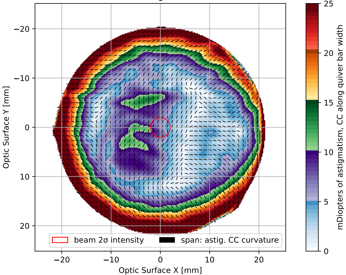
ZM4-SN1-110V astigmatism field in mD
