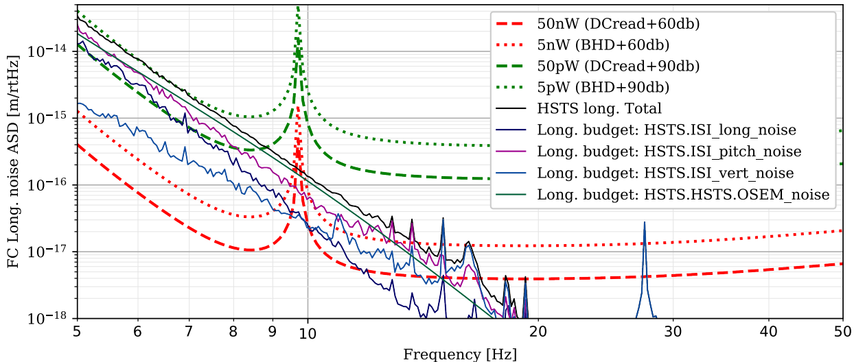
Figure 5: Length noise of a 300m FC with HSTS on standard aLIGO HAM ISIs (T1800066), with 3 mrad of vertical to length coupling, compared to length noise requirement imposed by back scattered light noise.
