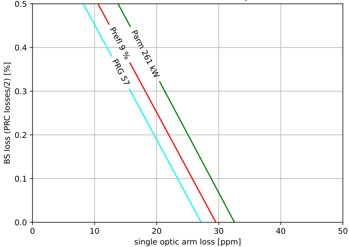
BS and arm losses contour comparison
