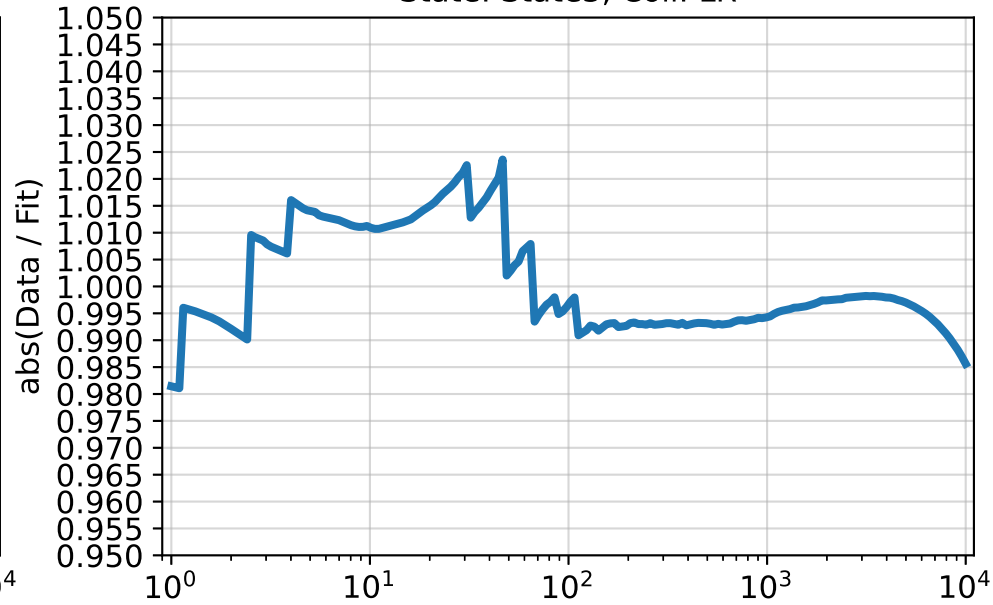
State: State3, Coil: LR
