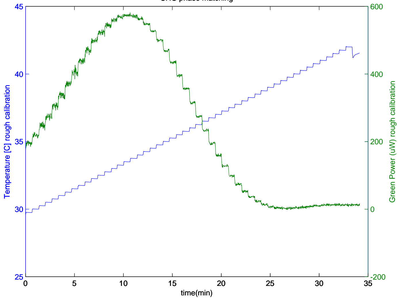
SHG phase matching
