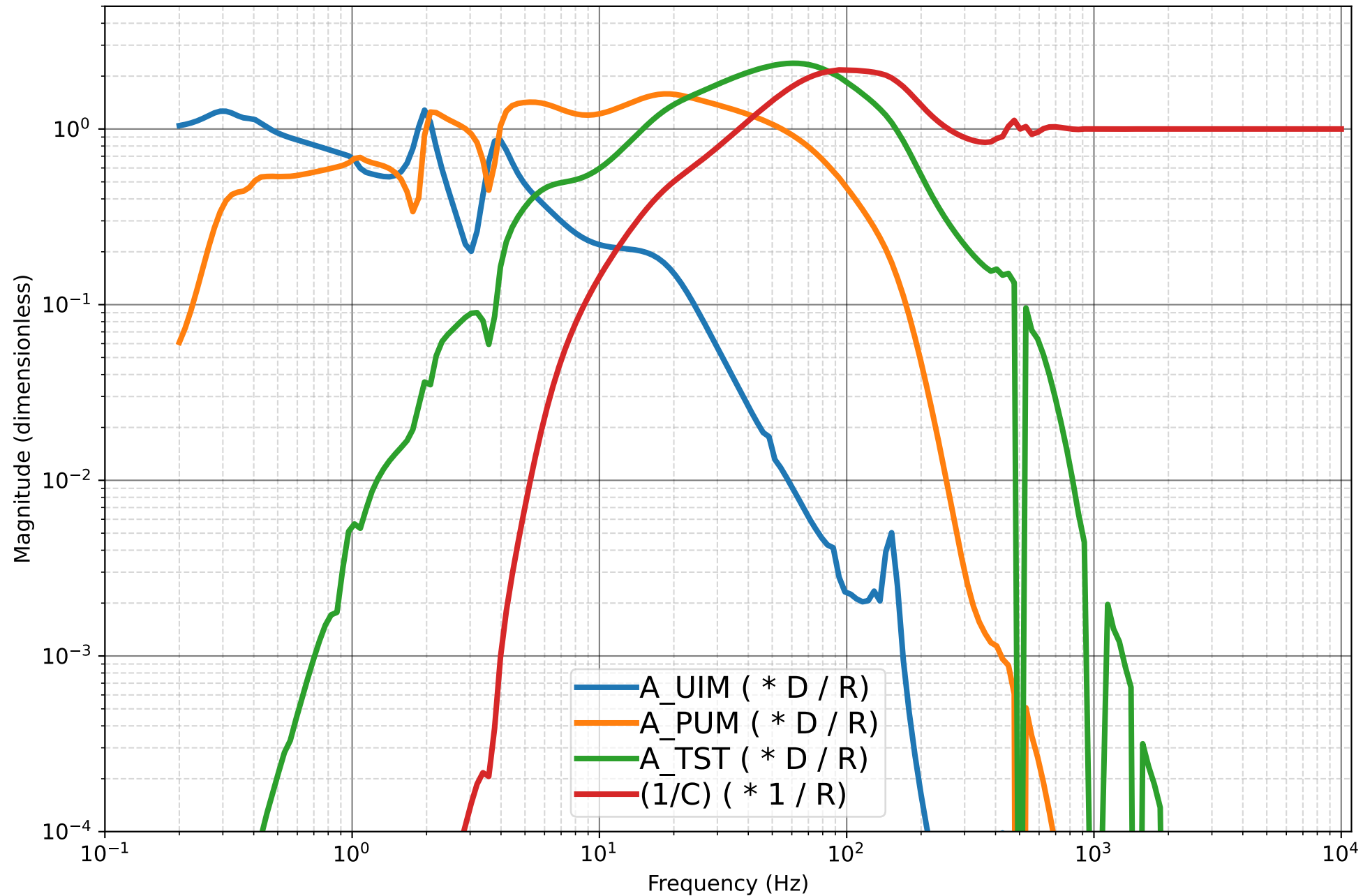
Post O3 [Post ITMY Swap] DARM Response, 2021-04-23 Relative Contribution of Actuator Stages and Sensing Function
