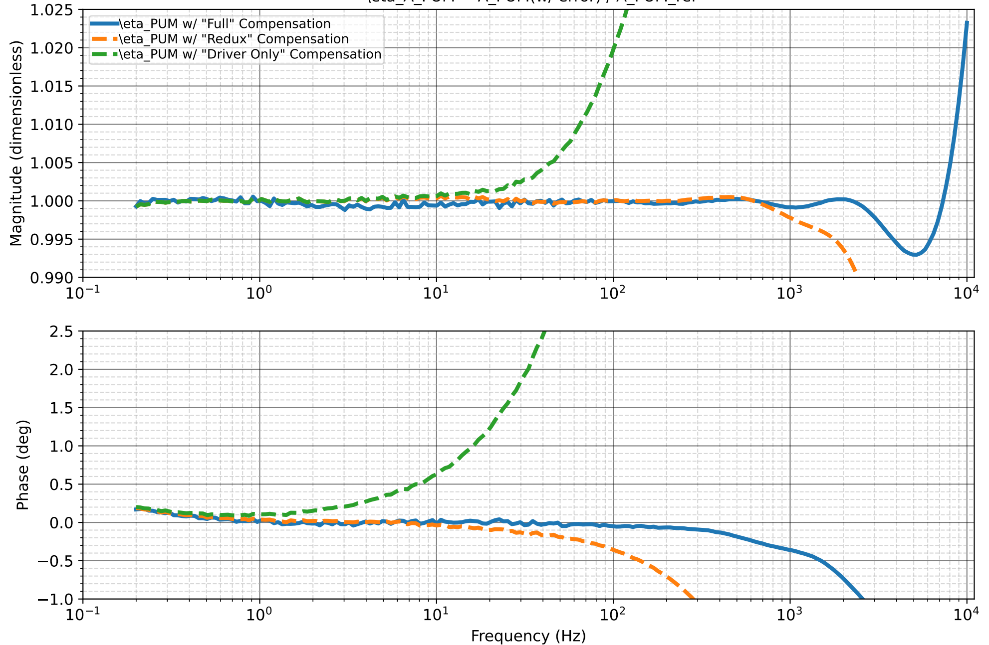
2022-01-14 H1 ETMX PUM State3 \eta_{A\_PUM} = A\_PUM(w/ \text{error}) / A\_PUM\_ref
