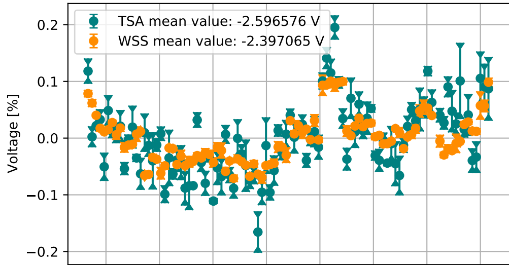
TSA Refl and WSS Tran Voltage
