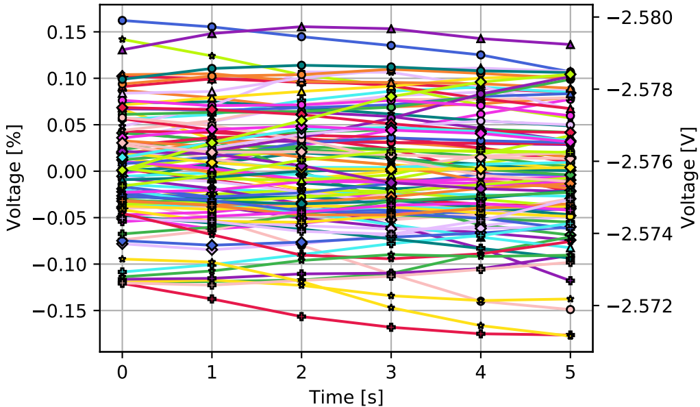
99 WSS Refl timeseries (overlaid)
