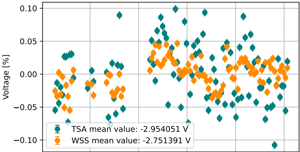
TSA Tran and WSS Refl Voltage
