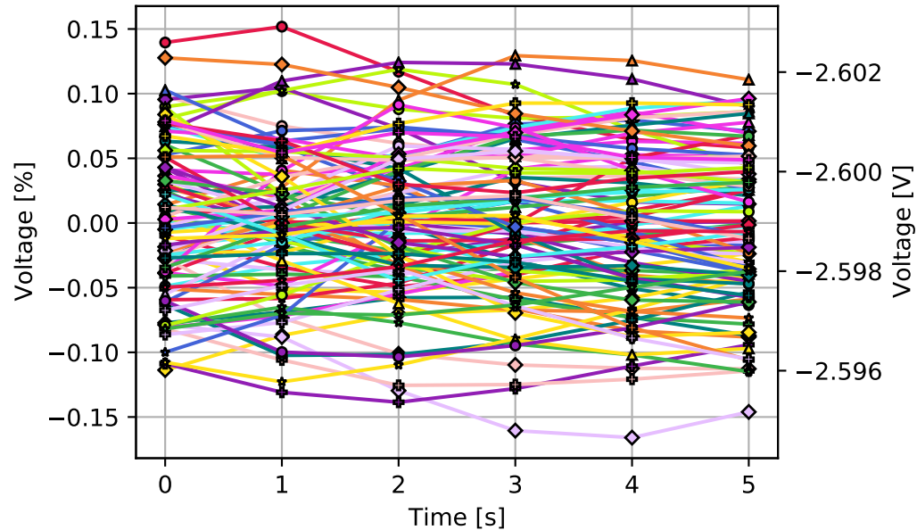
99 WSS Tran timeseries (overlaid)
