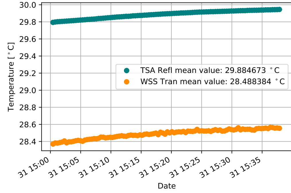
TSA Refl and WSS Tran Temperature
