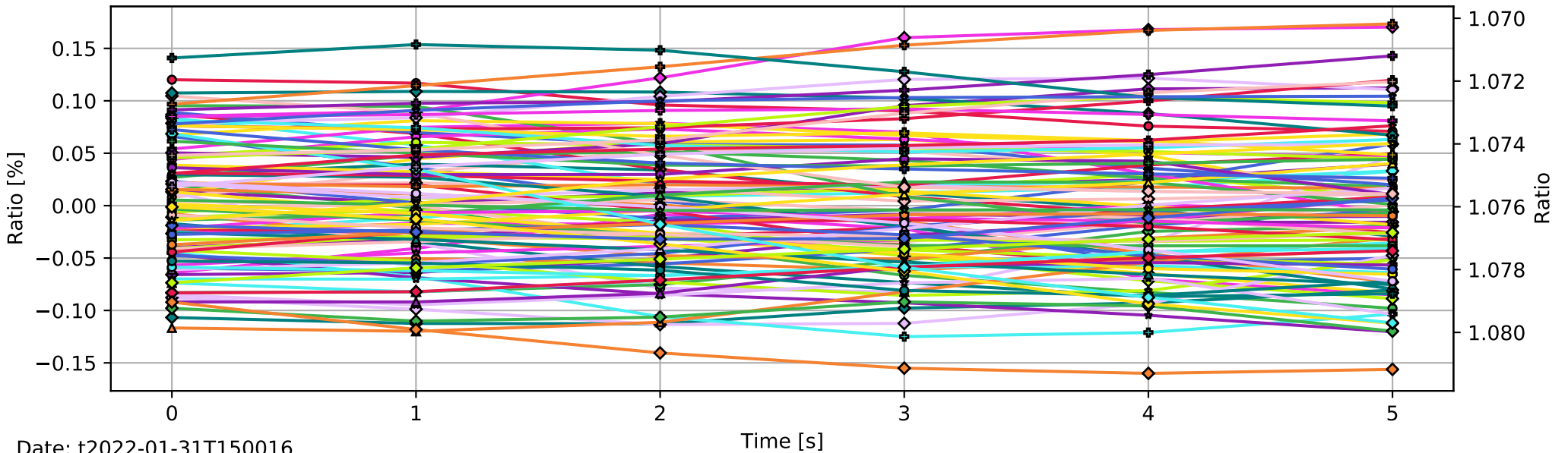
TSA Tran/WSS Refl timeseries ratios (overlaid)
