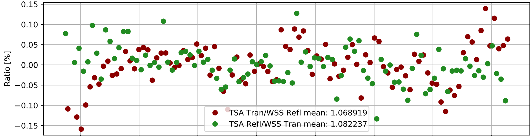
TSA/WSS timeseries ratios
