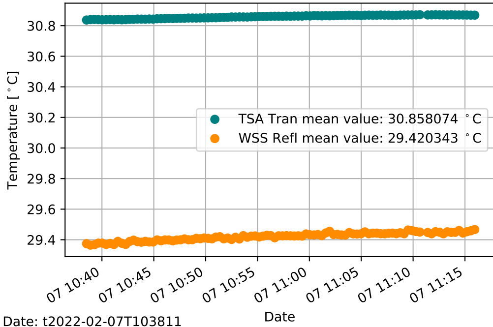
TSA Tran and WSS Refl Temperature
