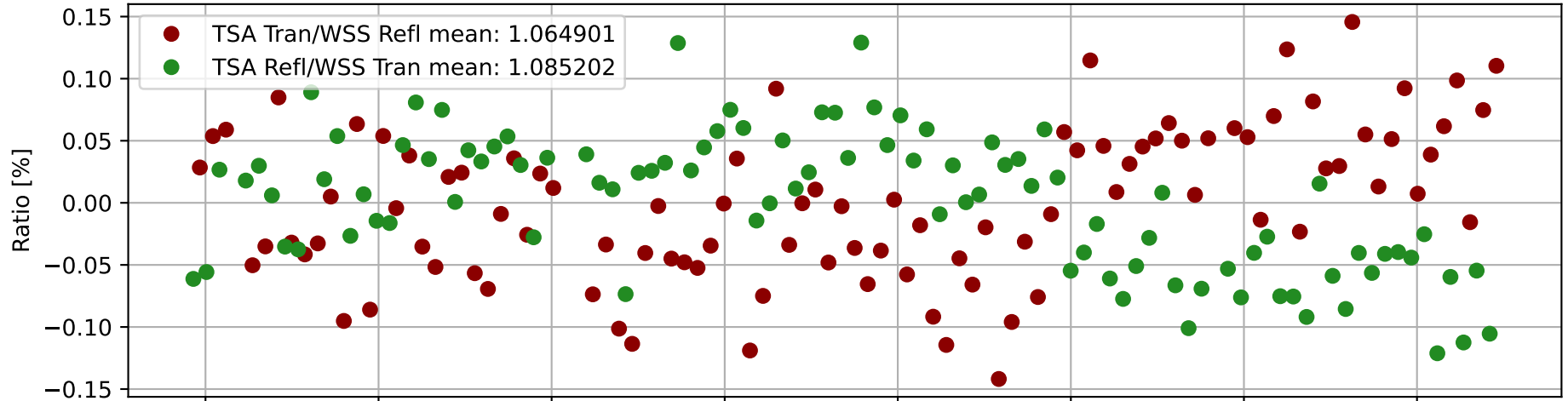
TSA/WSS final ratios
