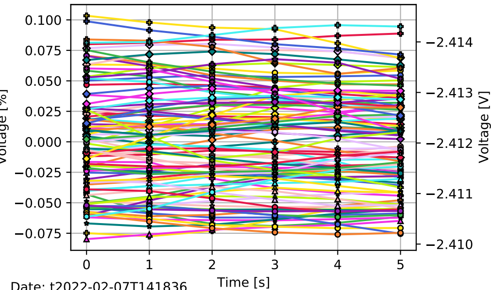
99 WSS Refl timeseries (overlaid)
