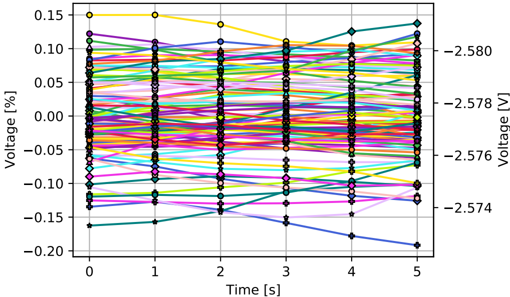
99 WSS Refl timeseries (overlaid)
