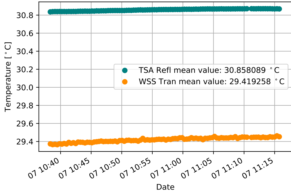
TSA Refl and WSS Tran Temperature
