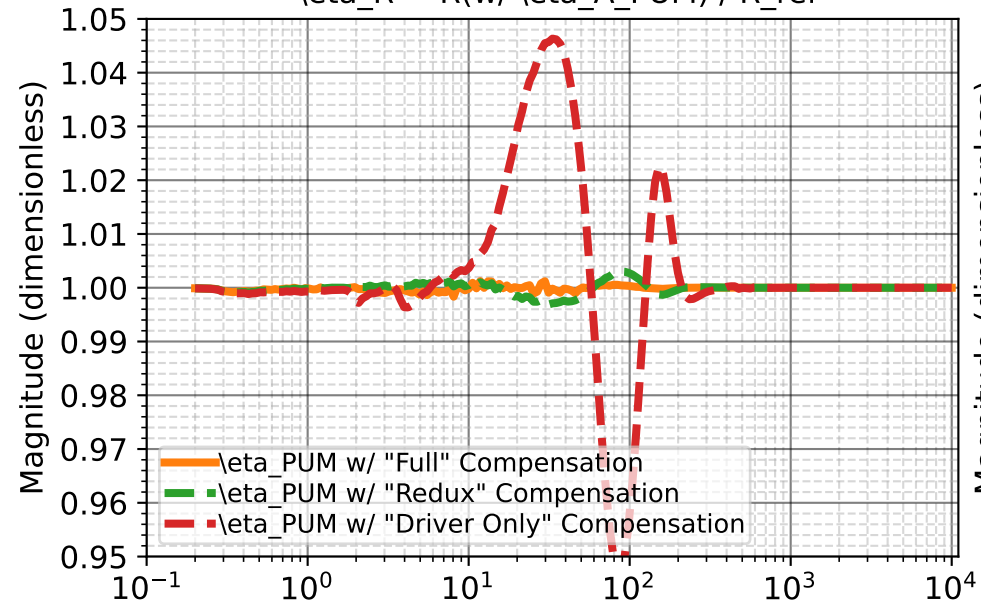
2022-01-10 H1 ITMX PUM State3 \eta_R = R(w/\eta_{A\_PUM}) / R_{ref}
