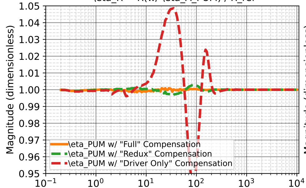
2022-01-11 H1 ITMY PUM State3 \eta_R = R(w/\eta_{A\_PUM}) / R_{ref}
