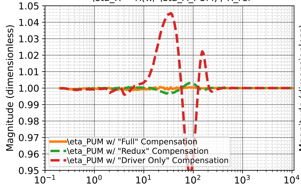
2022-01-14 H1 ETMX PUM State3 \eta_R = R(w/\eta_{A\_PUM}) / R_{ref}
