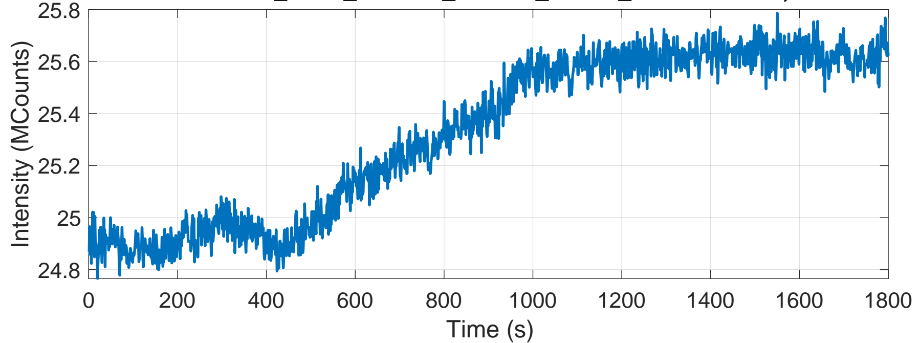
H1:TCS-ETMY_HWS_PROBE_TOTAL_PIXEL_VALUE.mean,s-trend
