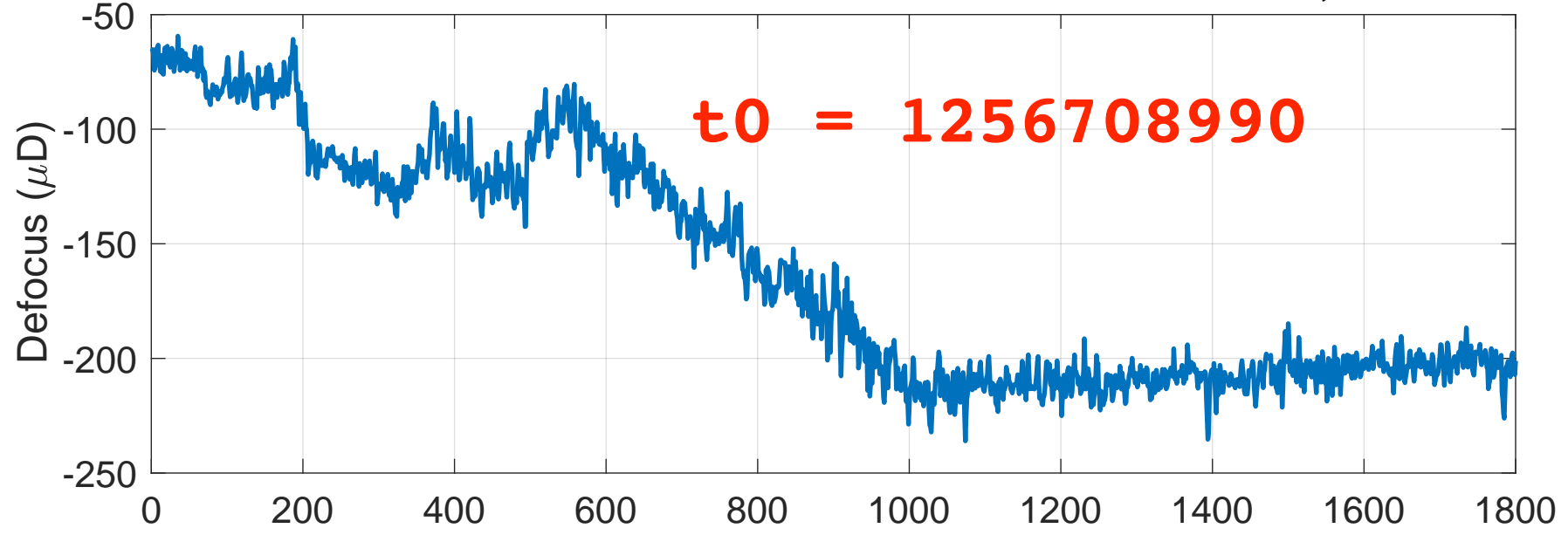
H1:TCS-ETMY_HWS_PROBE_SPHERICAL_POWER.mean,s-trend
