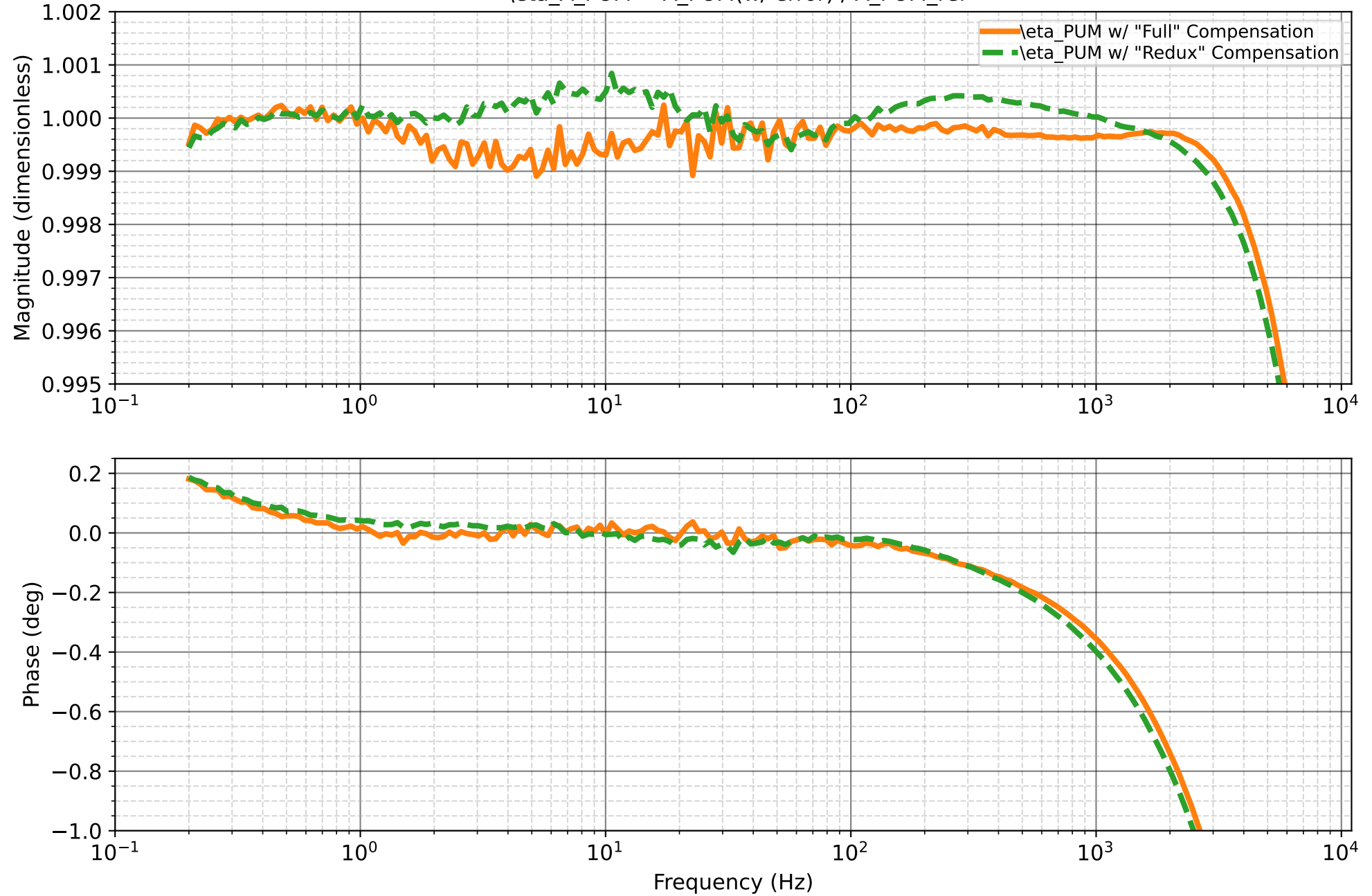
2022-01-14 H1 ETMX PUM State3 \eta_{A\_PUM} = A\_PUM(w/ error) / A\_PUM\_ref
