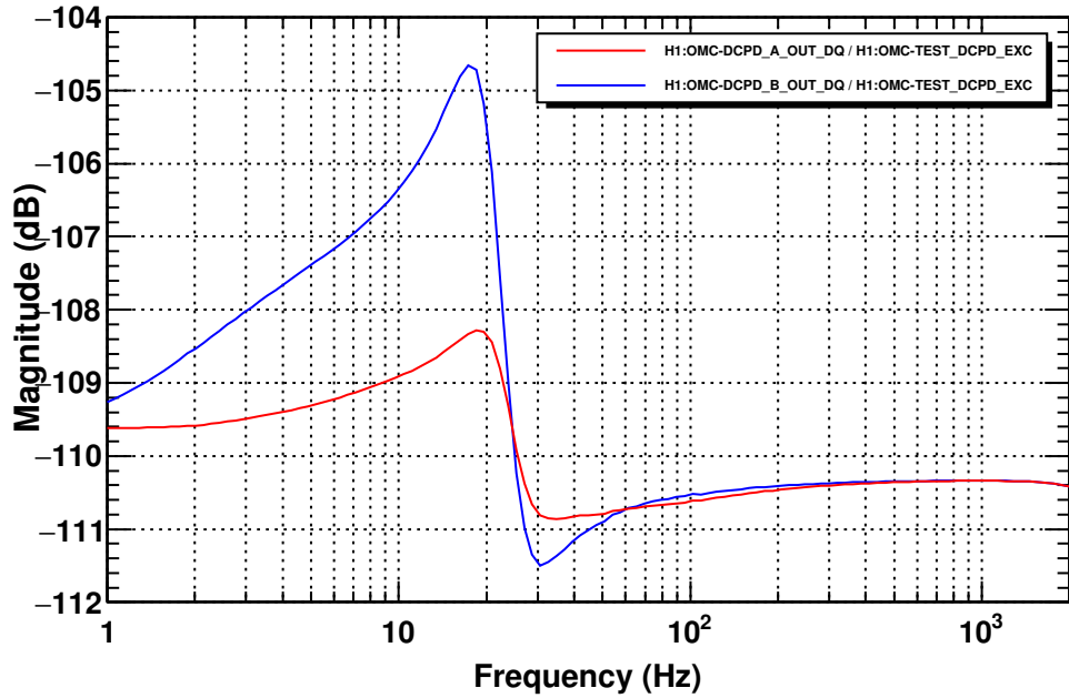
Transfer function
