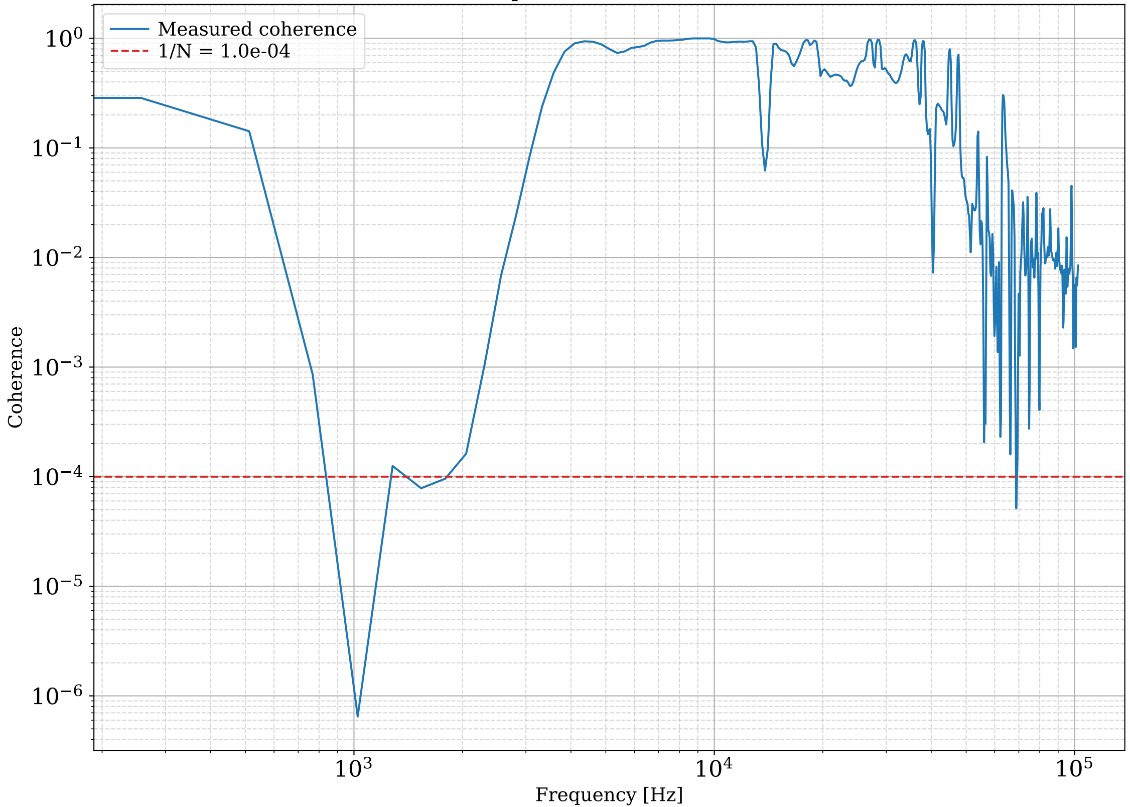
imc out2 iss second loop err2 coherence - 2022 03 15, 17:19:07
