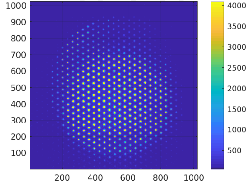
im1 = 1332039511_H1_ETMX_HWS_HS_Export.hdf5
