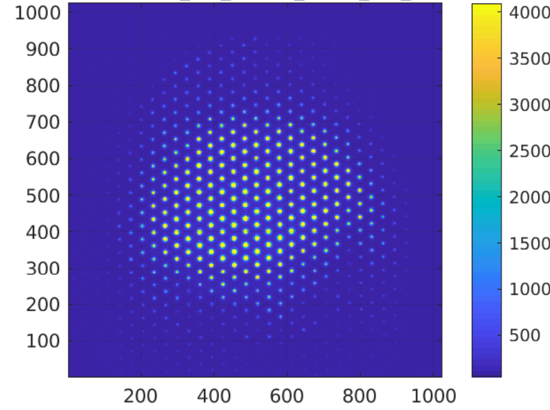
im2 = 1332050001_H1_ETMX_HWS_HS_Export.hdf5
