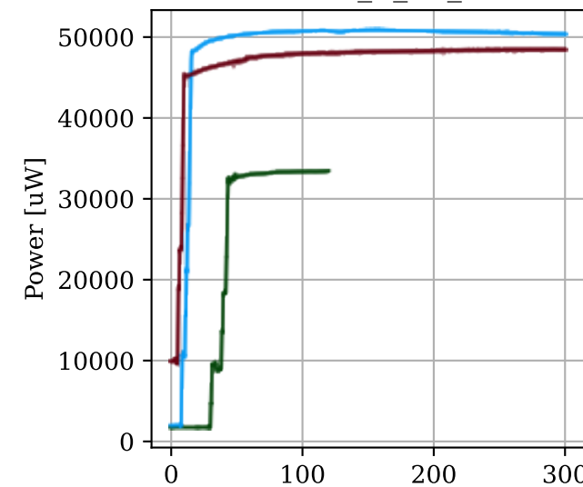
H1:ASC-Y_TR_B_NSUM_OUT16
