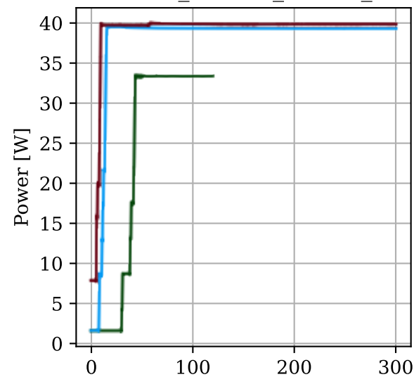
H1:ASC-X_TR_B_NSUM_OUT16
