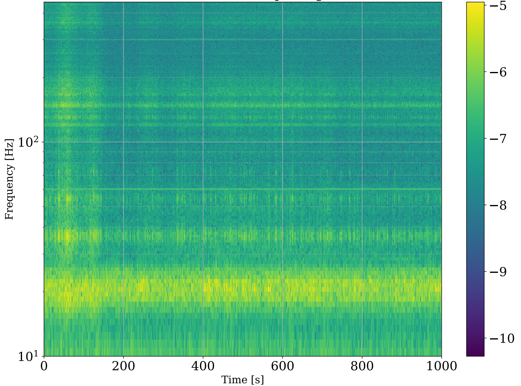
Uncalibrated DARM spectrogram
