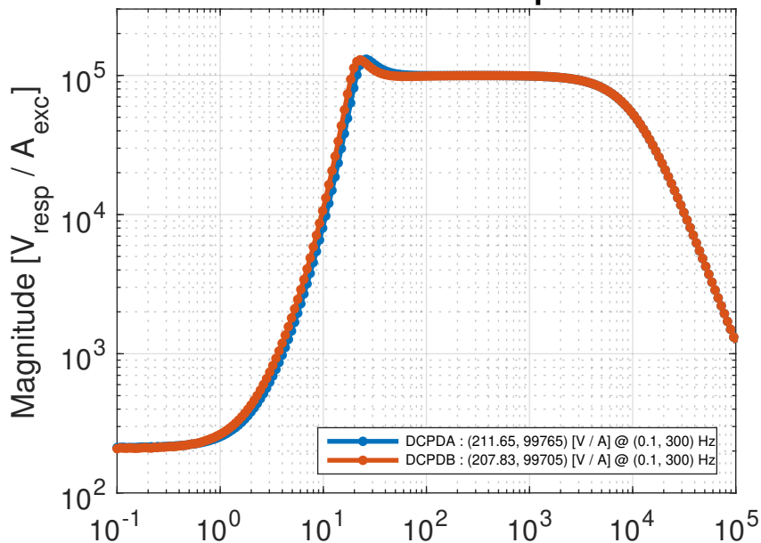
H1 OMC DCPD Transimpedance
