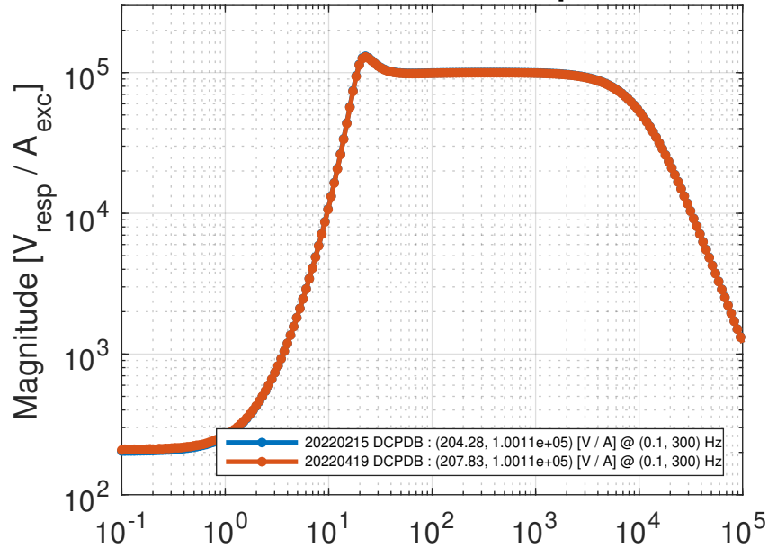
H1 OMC DCPD B Transimpedance
