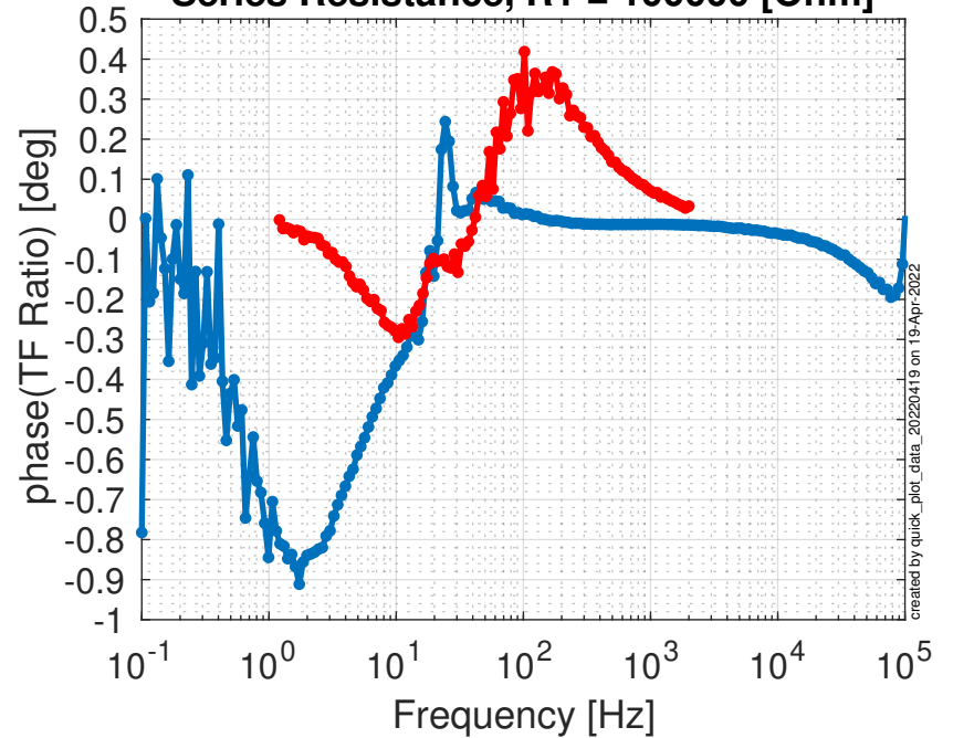
Series Resistance, R1 = 100000 [Ohm]
