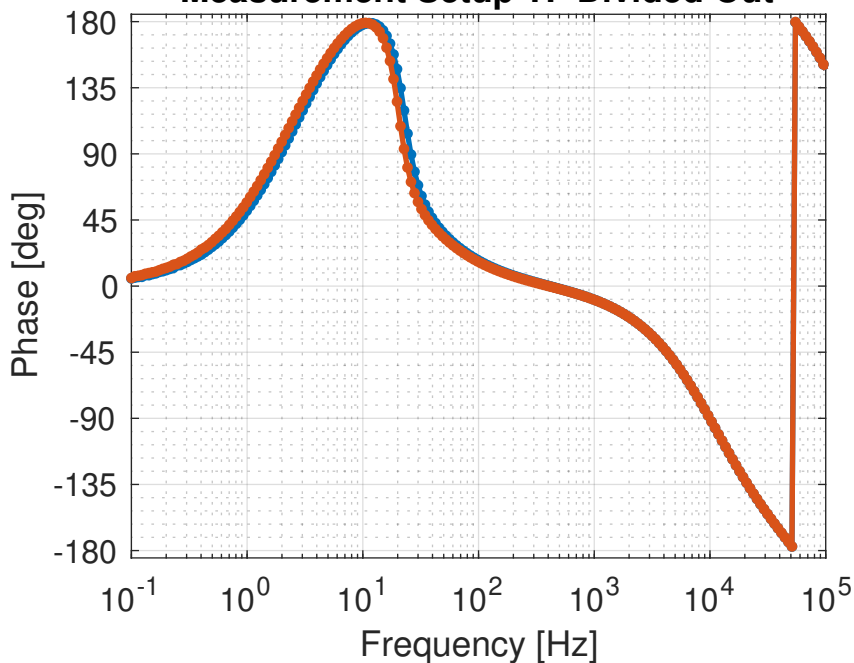
Measurement Setup TF Divided Out
