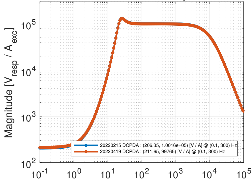
H1 OMC DCPD A Transimpedance
