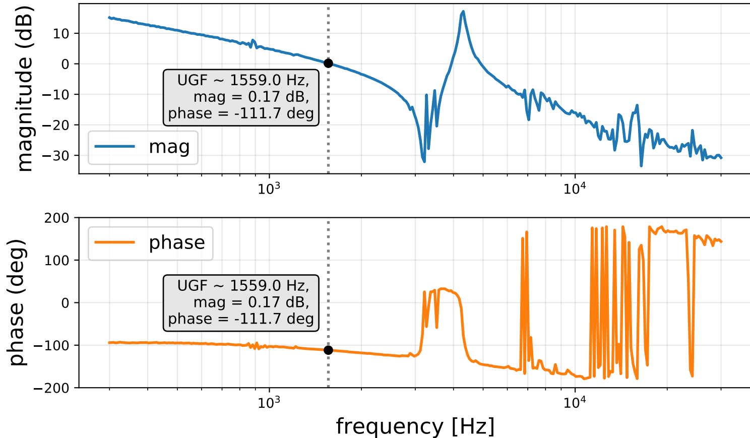
OPO PZT 1 transfer function, SR785 measured 4/22/22
