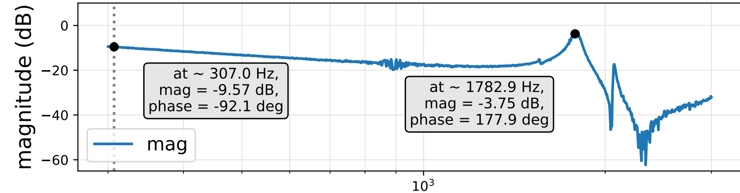
OPO PZT 2 transfer function, SR785 measured 4/27/22
