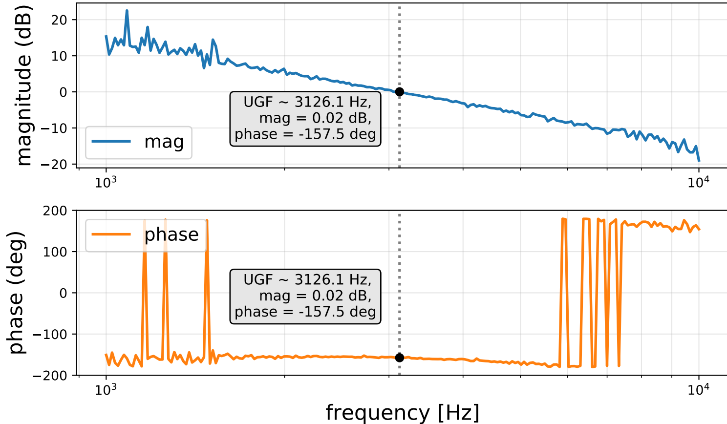
CLF (no RLF) transfer function, SR785 measured 4/27/22
