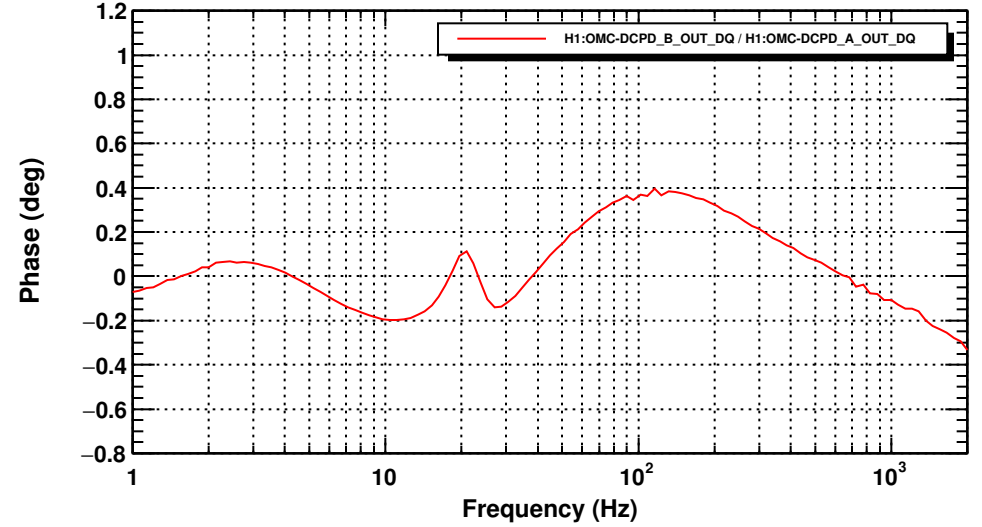
Transfer function
