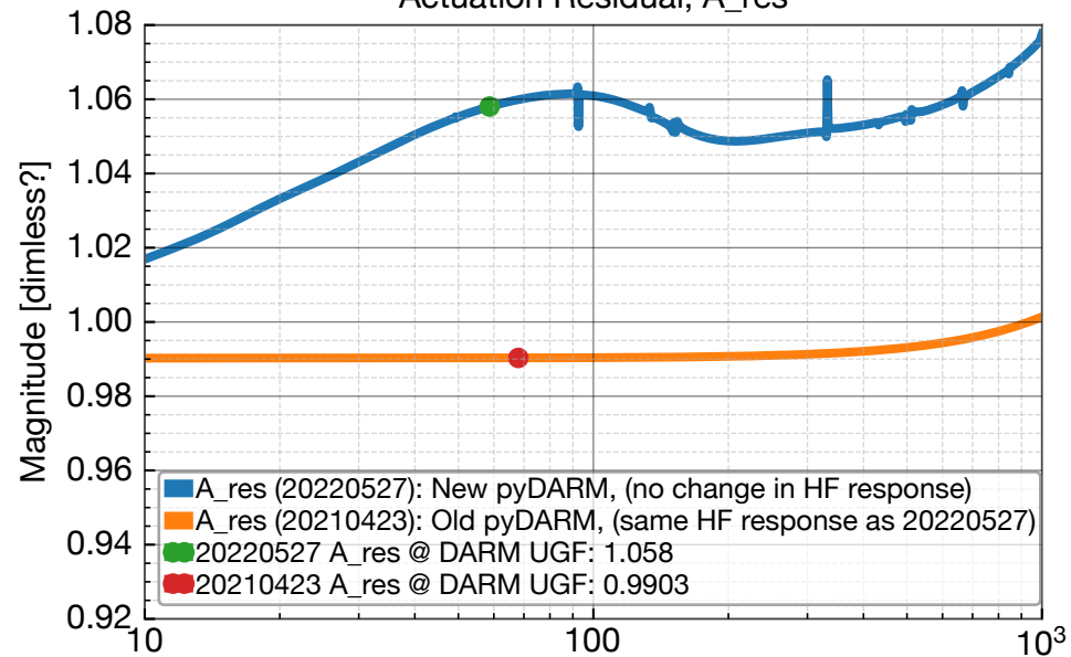
20210423 DARM UGF: 68.0507 [Hz]
