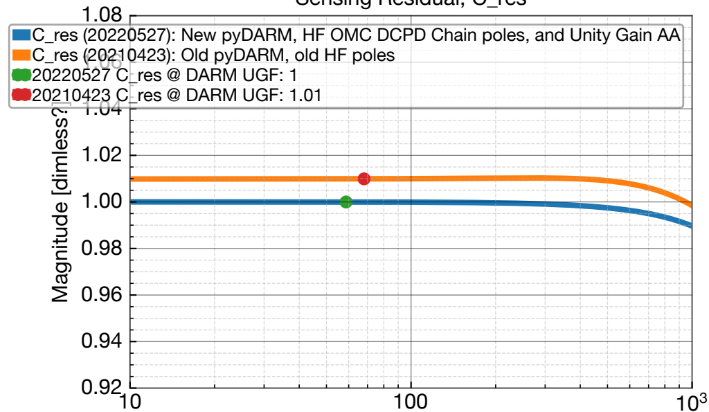
20220527 DARM UGF: 58.7177 [Hz]
