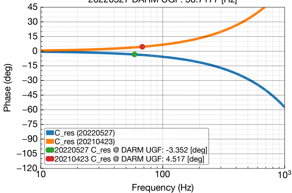
20220527 DARM UGF: 58.7177 [Hz]
