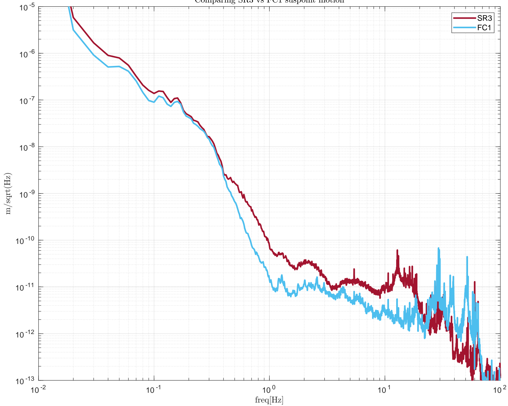
Comparing SR3 vs FC1 suspoint motion
