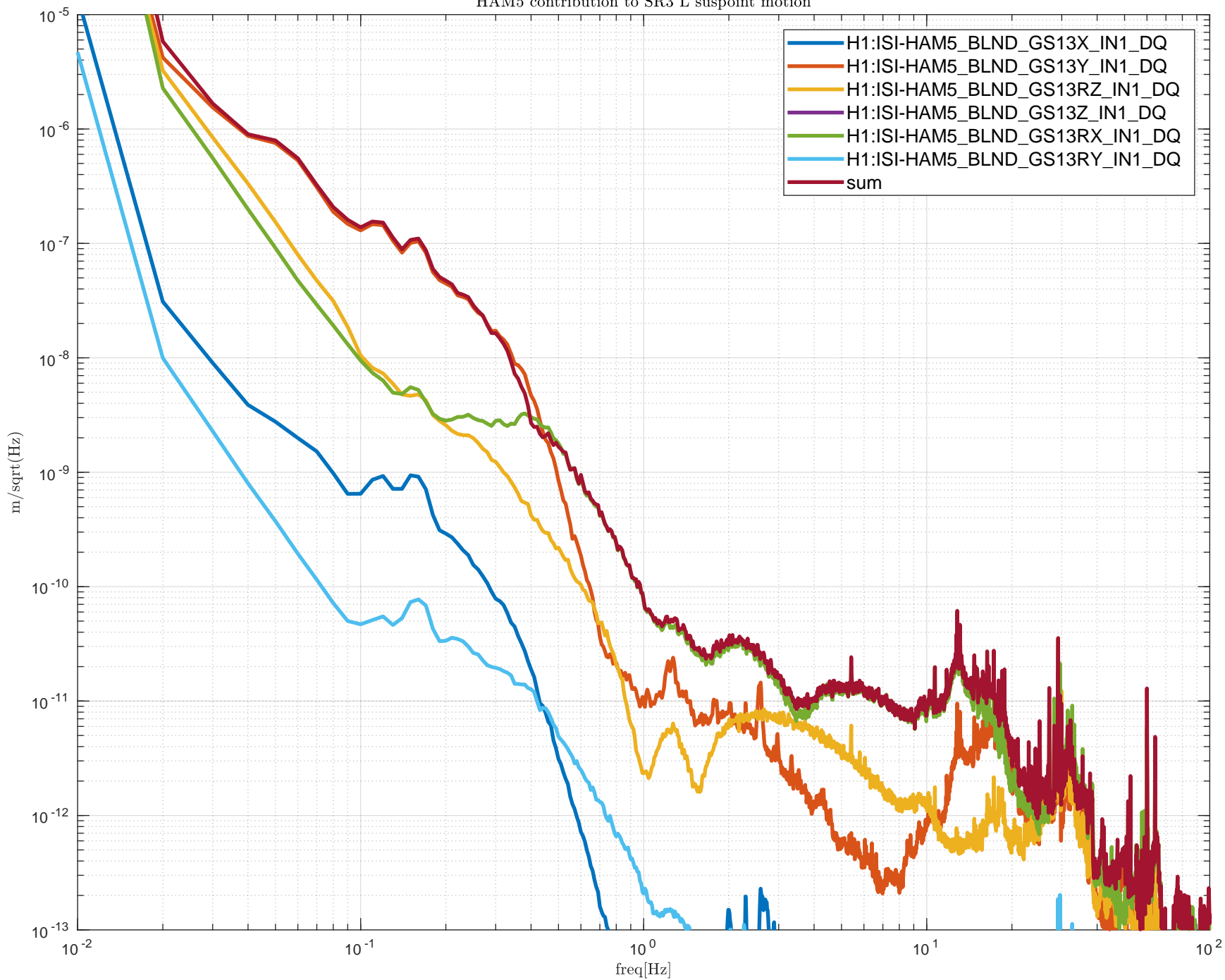
HAM5 contribution to SR3 L suspoint motion
