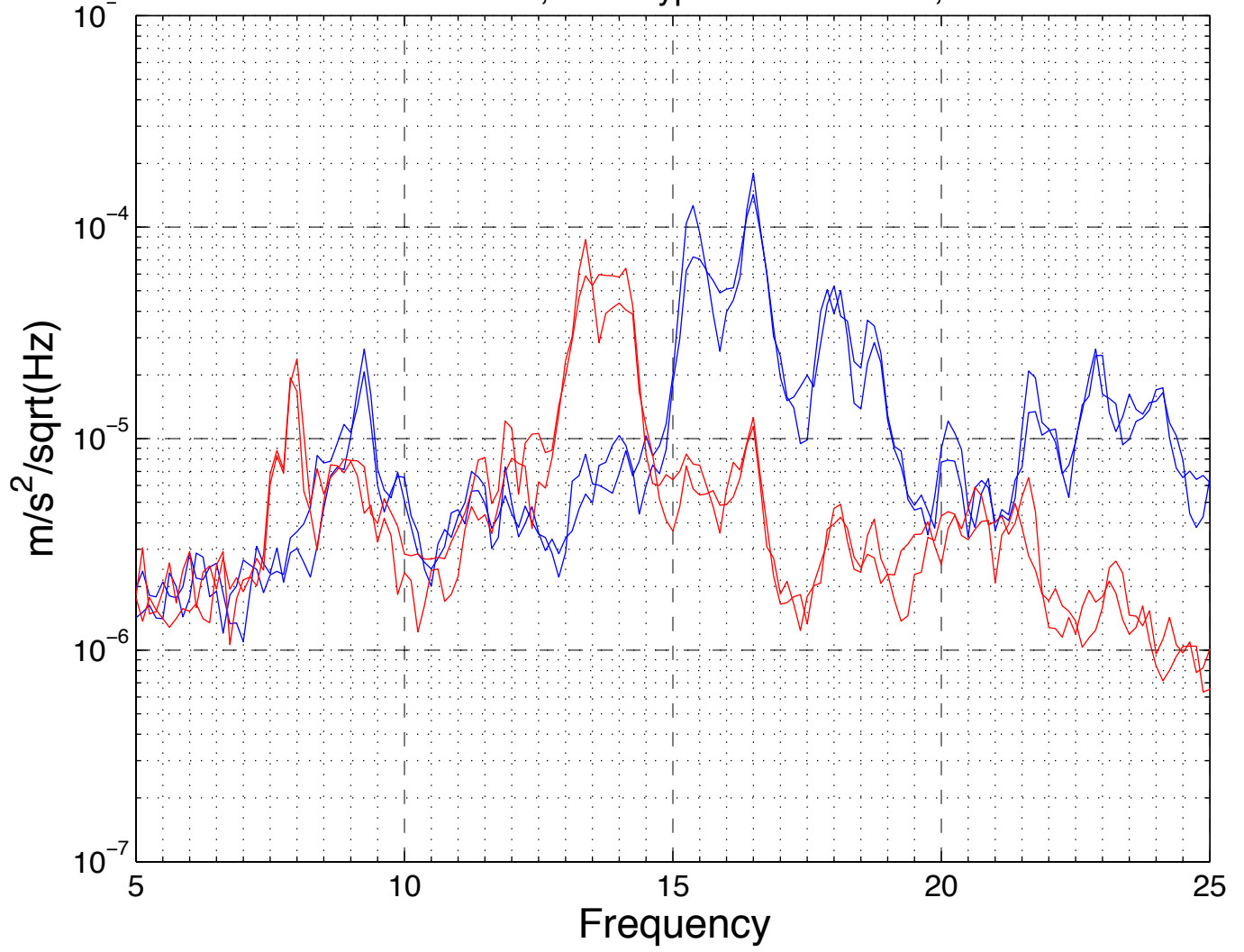
Beam direction Acceleration, RED: typical 39m section, BLUE: 33.5m section
