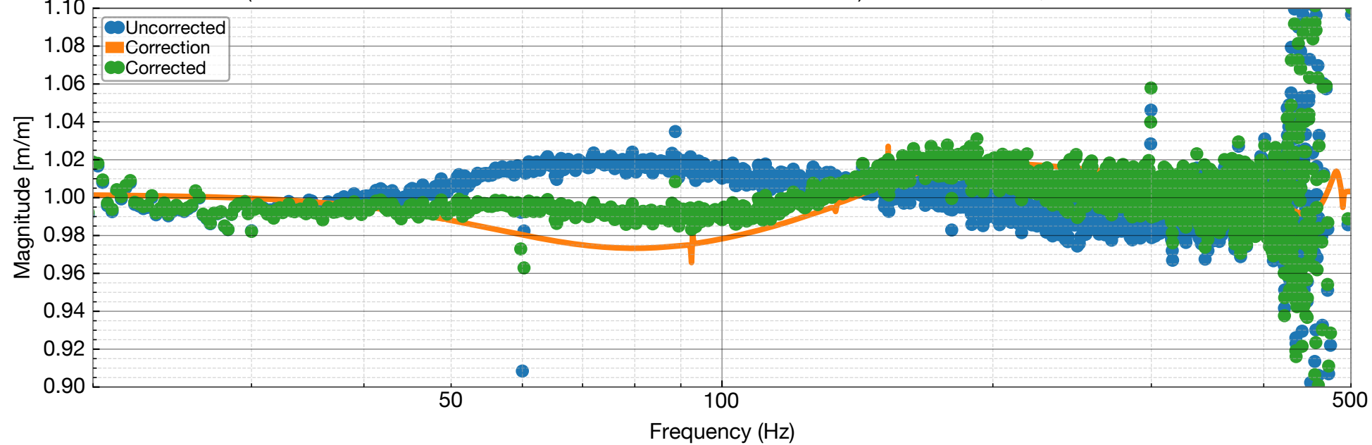
(CAL-DELTA_EXTERNAL_DQ / CAL-PCALY_RX_PD_OUT_DQ) Transfer Function, and Corrections
