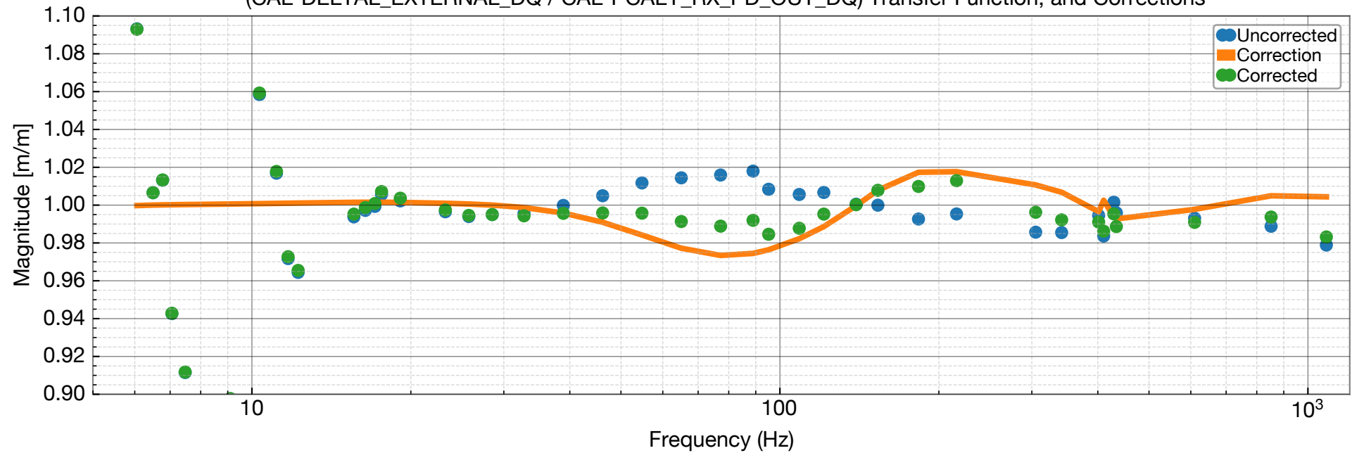
(CAL-DELTA_EXTERNAL_DQ / CAL-PCALY_RX_PD_OUT_DQ) Transfer Function, and Corrections
