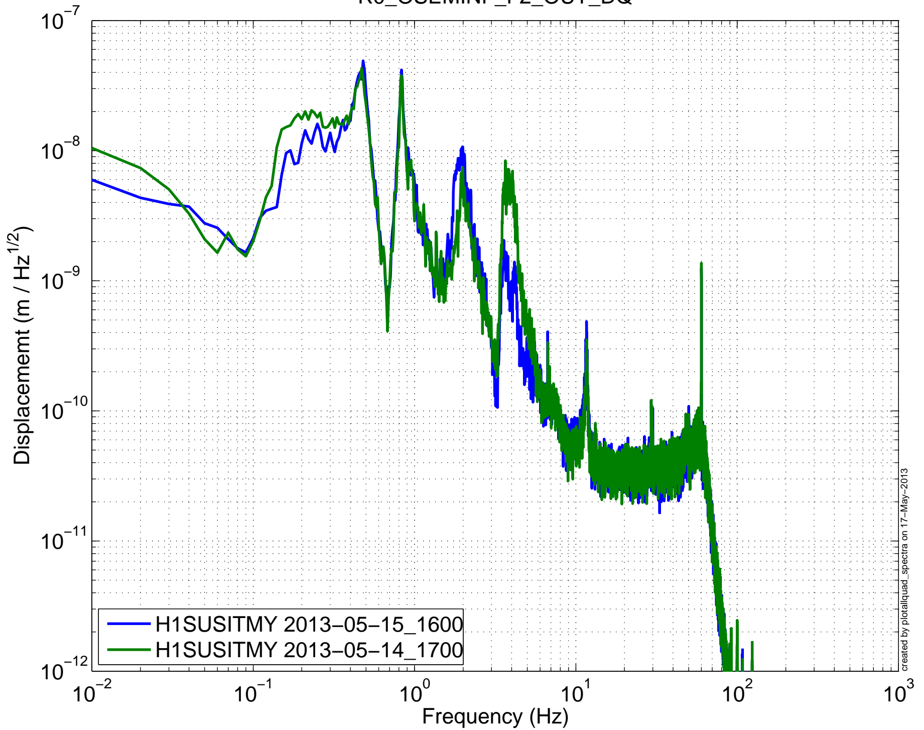
(QUAD) Amplitude Spectral Density – Damping ON R0_OSEMINF_F2_OUT_DQ
