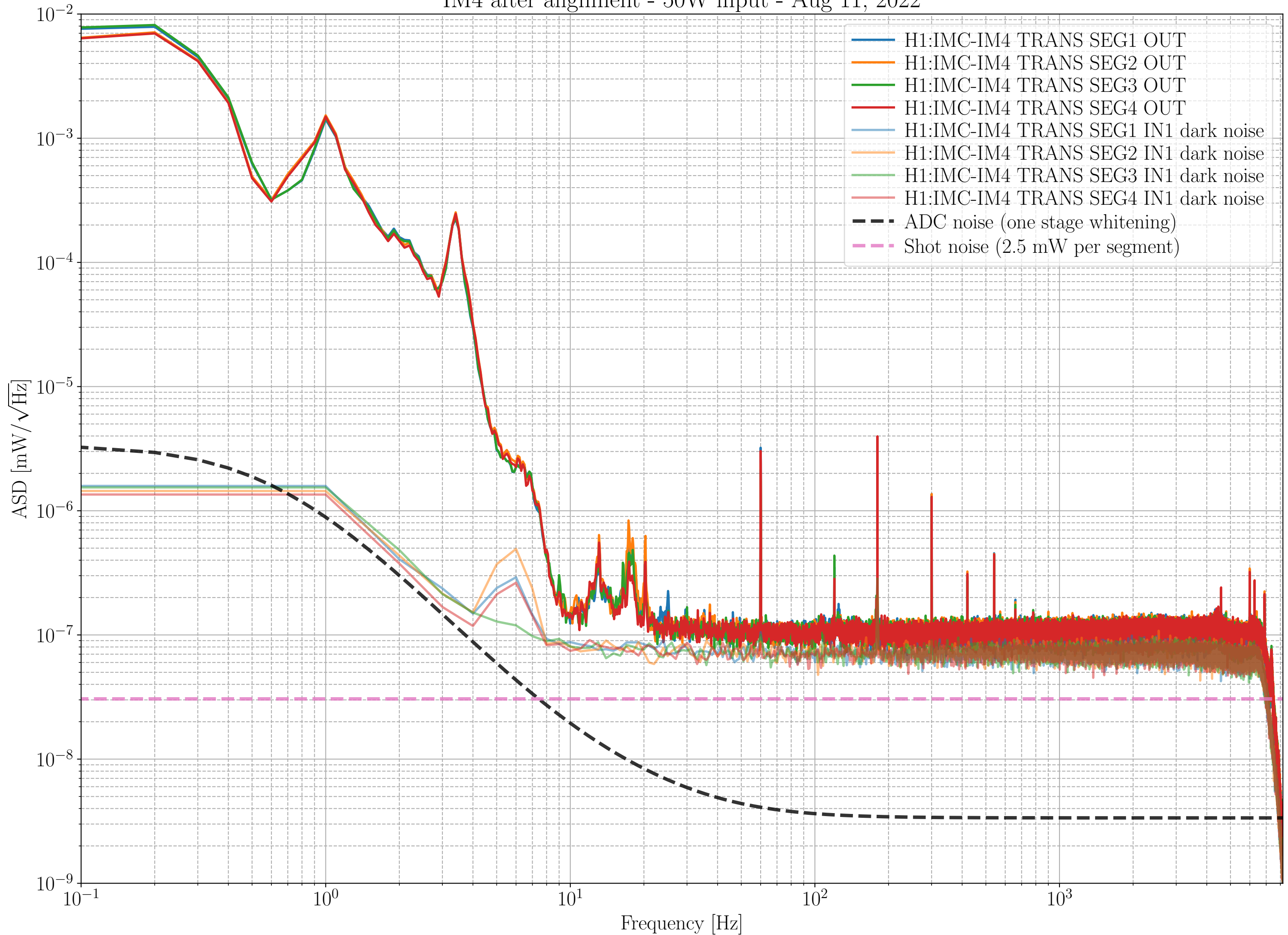
IM4 after alignment - 50W input - Aug 11, 2022
