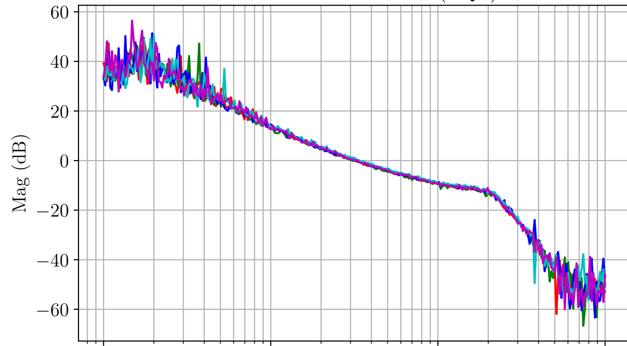
LO Transfer Functions (SQZ)
