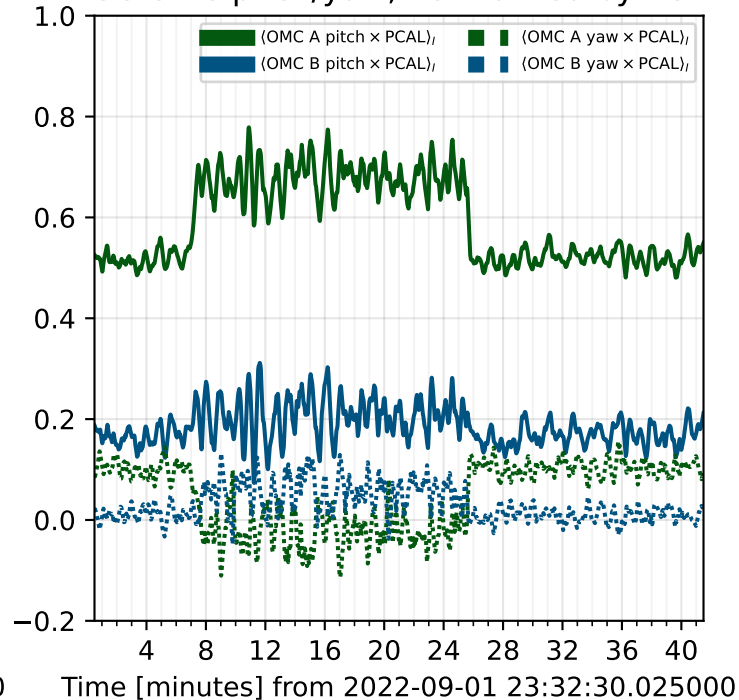
ASC OMC pitch/yaw, normalized by PCAL
