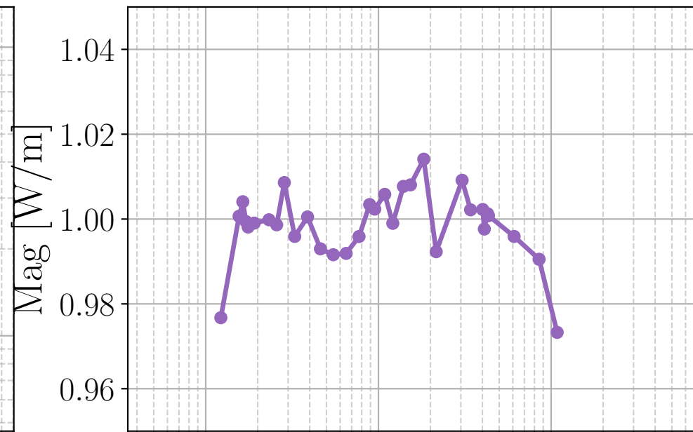
Residuals
