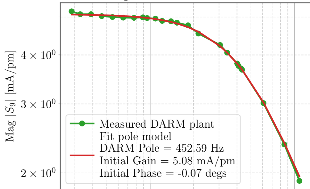
DARM plant measurement vs model
