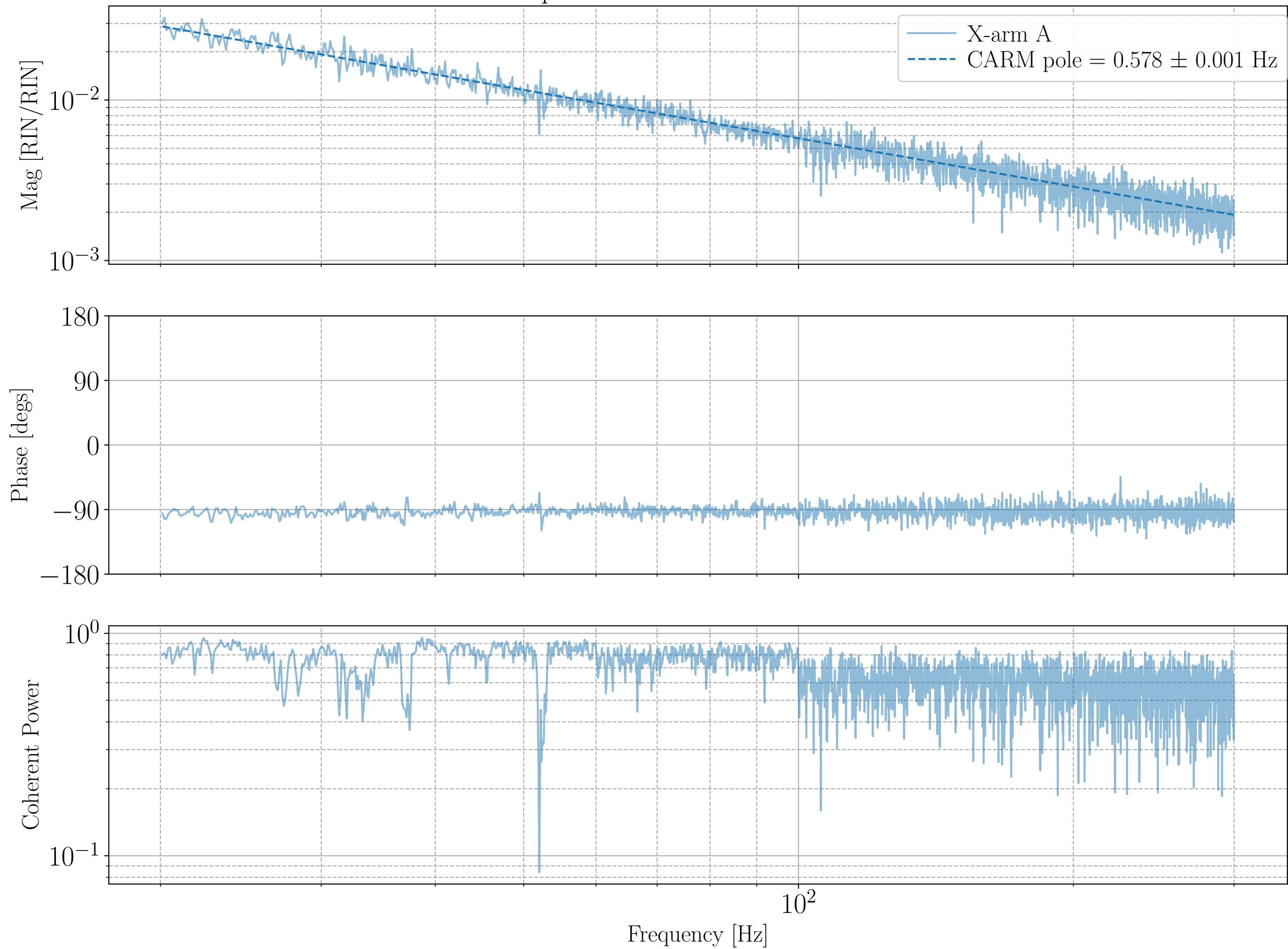
Input RIN to X-arm A RIN fits
