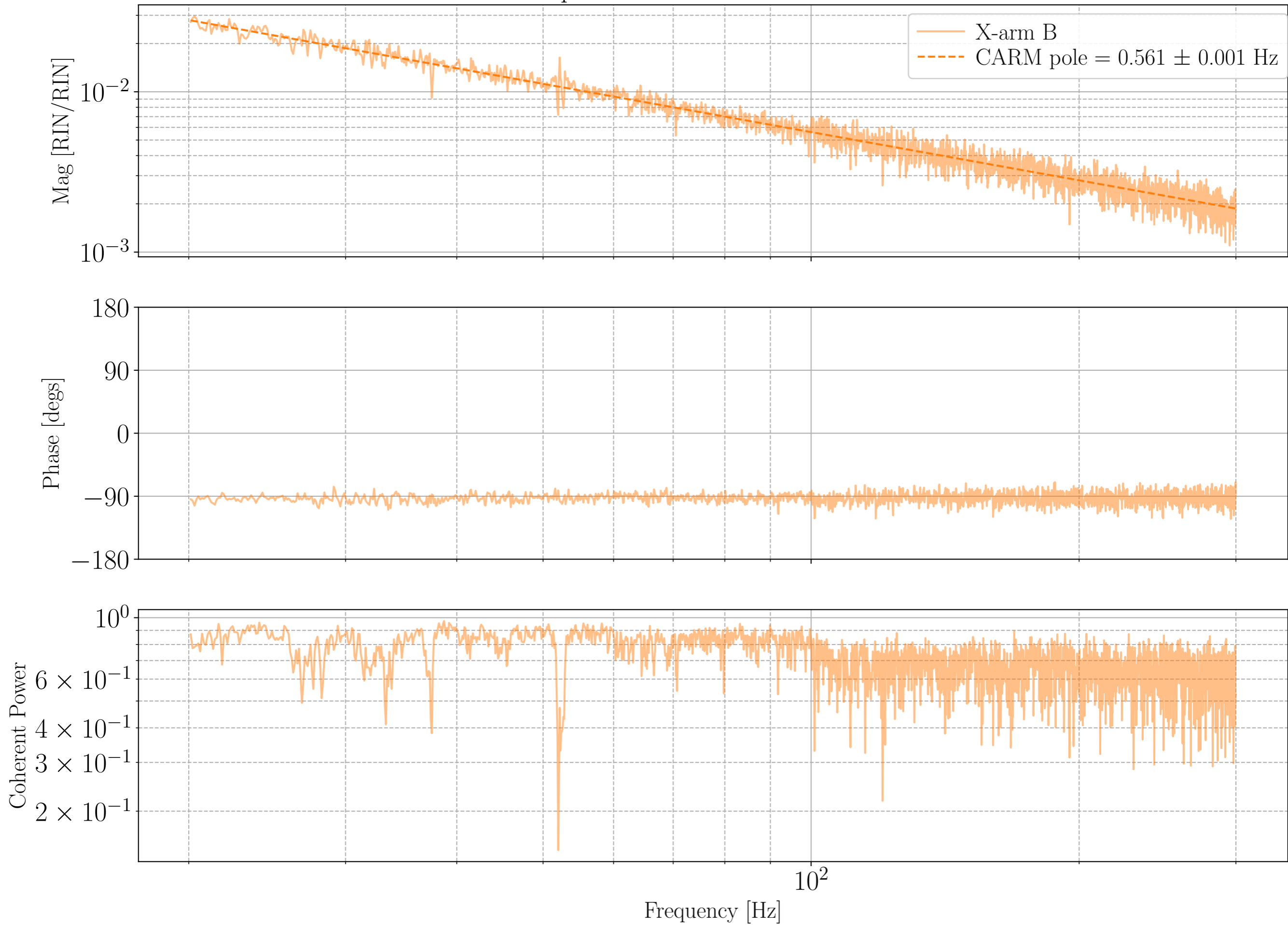
Input RIN to X-arm B RIN fits
