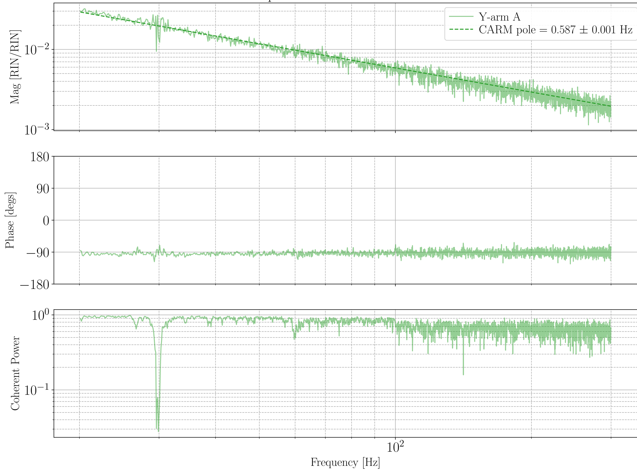
Input RIN to Y-arm A RIN fits
