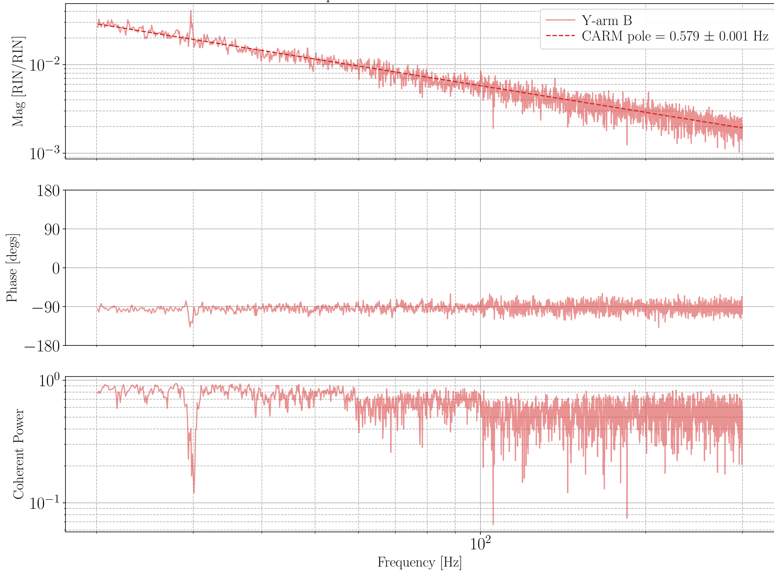
Input RIN to Y-arm B RIN fits
