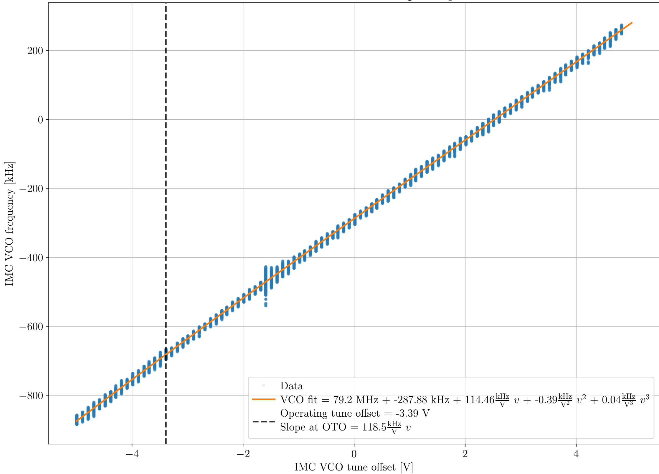
IMC VCO tune offset voltage sweep
