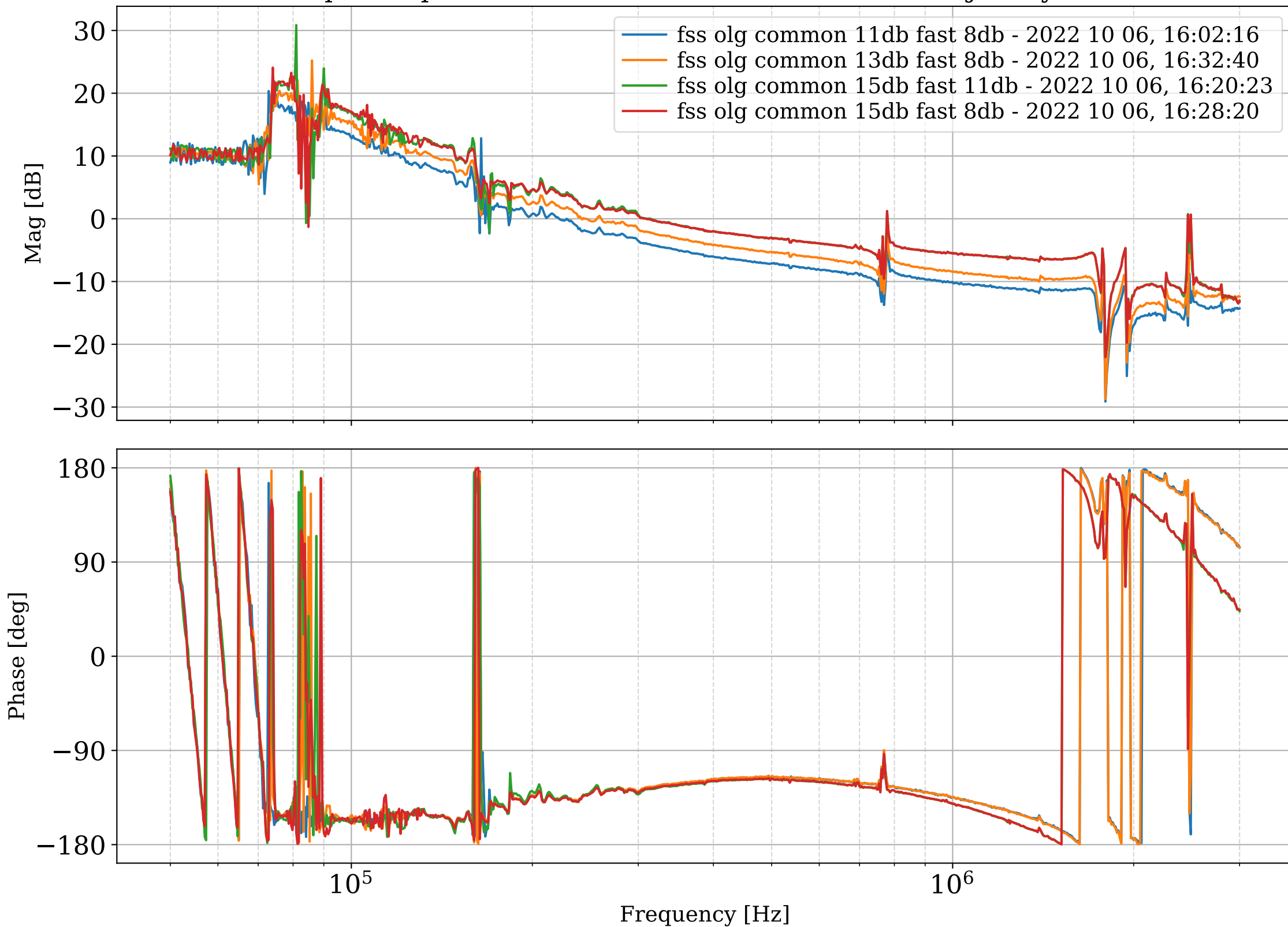
FSS open loop transfer functions - October 6 2022 - adjust by +10 dB
